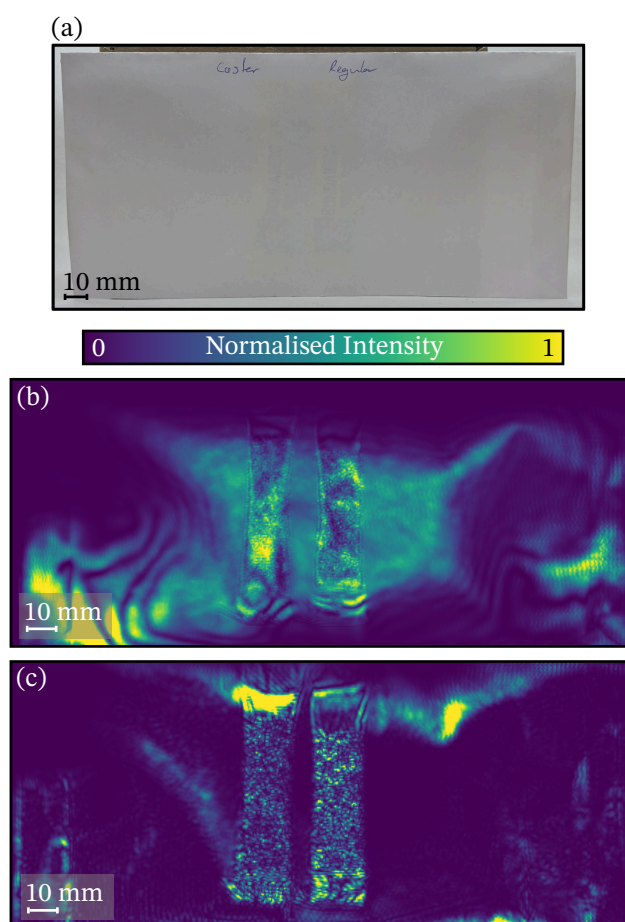
Figure 3.9: Detection of concealed granular substance in paper envelope. (a) Photograph of the envelope, with the sachets containing caster and regular sugar slightly visible through the paper. (b) Bright-field time domain image of the envelope. (c) Dark-field time domain image of the envelope. The smaller grain size of the caster sugar scatters less terahertz power, as is evident in the dark-field image. We clip both images to the central 98% intensity distribution of data to remove any outliers.
