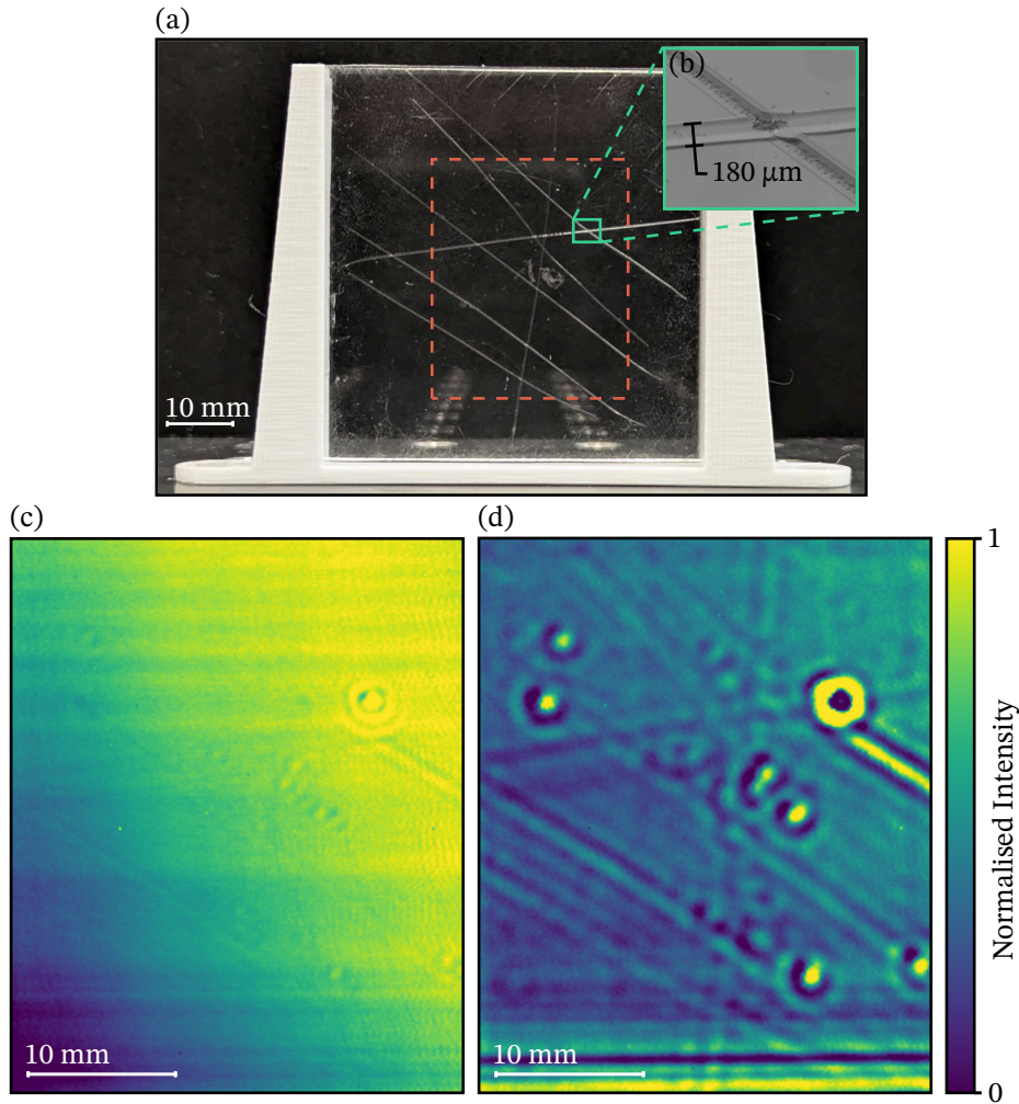
Figure 3.6: Detection of surface defects on acrylic substrate. (a) Photograph of the acrylic slab with several surface scratches. (b) Optical micrograph of surface defect, indicating the scratch defects are approximately 180\text{ }\mu\text{m} in width. (c) Bright-field time domain image. (d) Dark-field time domain image. We clip both images to the central 98% intensity distribution of data to remove any outliers.
