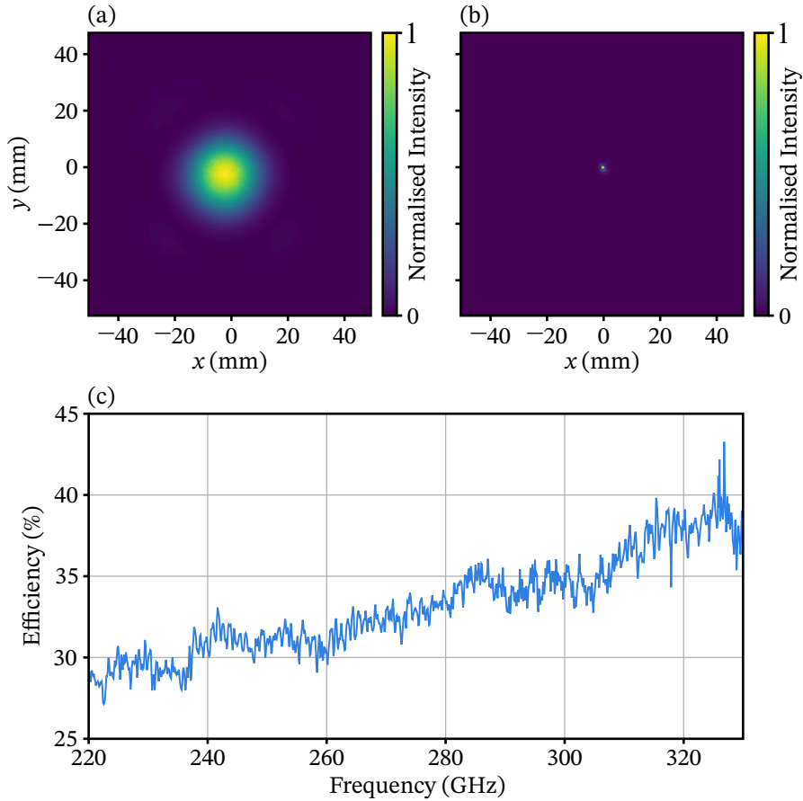
Figure 3.4: Power transmission efficiency of the optical train. (a) Transmission intensity at 275 GHz, measured 100 mm away from the horn antenna, without the dark-field system. (b) Transmission intensity at 275 GHz, measured at the focal plane of the dark-field system. (c) Percentage transmission efficiency at the focal plane relative to the horn antenna.
