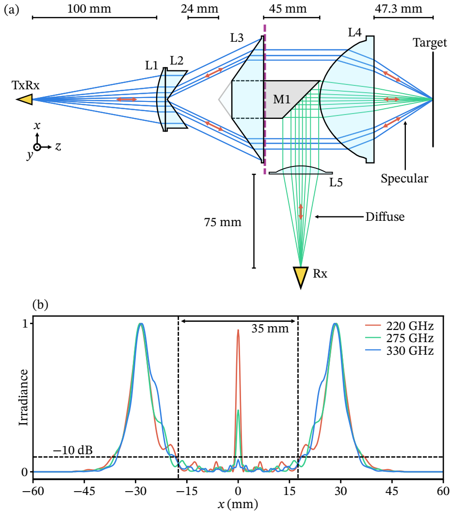
Figure 3.1: Lens train model of the imaging system. (a) Lens diagram showing the path from the transceiver to the target through L1: Horn collimating lens; L2: Diverging axicon lens; L3: Collimating axicon lens; L4: Objective lens M1: 45^\circ mirror; L5: Collector collimating lens. (b) Cross section of collimated annular-beam, indicated by the purple dashed line, with 24 mm axicon separation, computed with the Physical Optics Propagation mode in ANSYS Zemax OpticStudio. All three frequencies have at least 36 mm centre null diameter at -10 dB.
