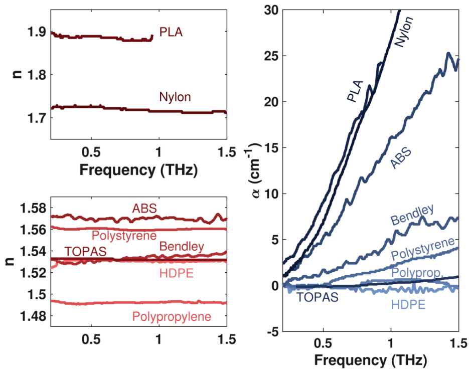
Figure 1.15: Refractive index and absorption coefficient of various thermoplastics used in FDM 3D-printing. The acronyms and abbreviations are HDPE = High Density Polyethylene, Polyprop. = Polypropylene, ABS = Acrylonitrile Butadiene Styrene, and PLA = Polylactic acid. Data from Refs. [138] and [137]. Reprinted from [139] with permission from AIP Publishing.
