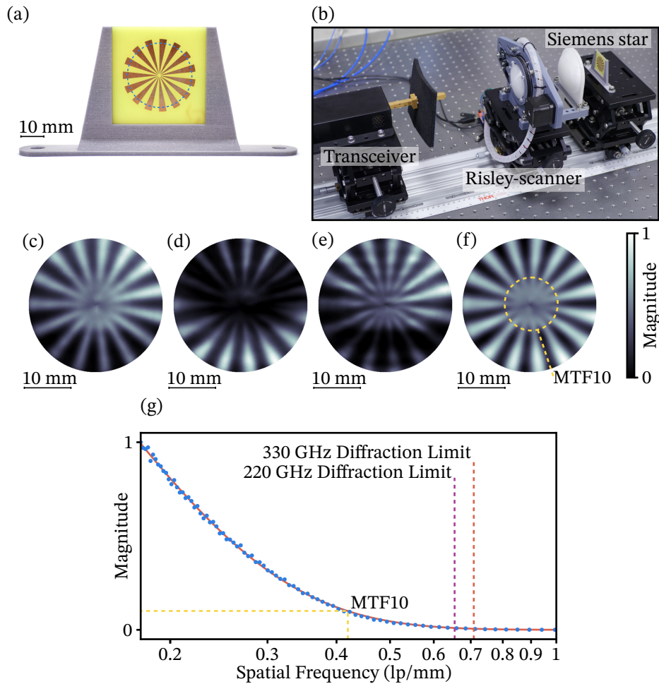
Figure 2.8: Evaluation of the spatial resolution of the imaging system using a Siemens star imaging target. (a) Front view photo of Siemens star. (b) Photo of experimental setup. (c, d, e) S_{11} at 220, 275 and 330 GHz. (f) Observation plane at the peak reflection in the time-domain. (g) Modulation transfer function of the imaging system, extracted from the observation plane. 10% contrast occurs at 0.419 lp/mm.
