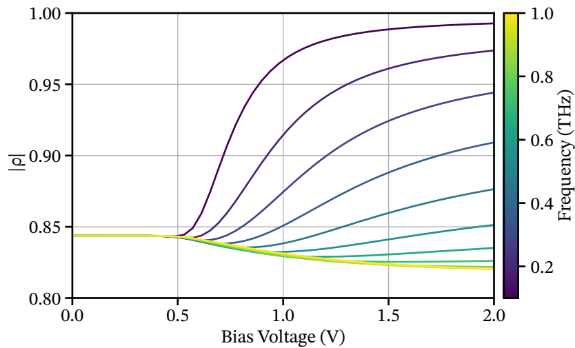
Figure 4.2: Change in reflectivity of modelled material between 0.1–1 THz. Fresnel reflectivity coefficient for a normally incident wave incident upon the material modelled by Fig. 4.1(b) and (c), referenced to a refractive index of 1.
