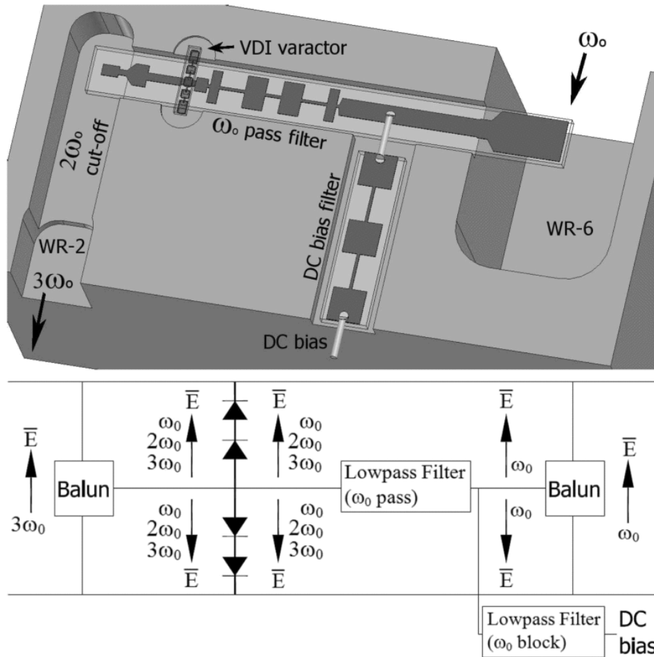
Figure 1.10: Sketch and schematic of a 440 GHz frequency tripler, based on Virginia Diodes (VDI) Schottky varactor diode chip. The waveguide block is split in the E-plane and the top half removed to expose the circuits. The waveguide backshorts are machined in a fixed position. Adapted from [67] © 2007 IEEE.
