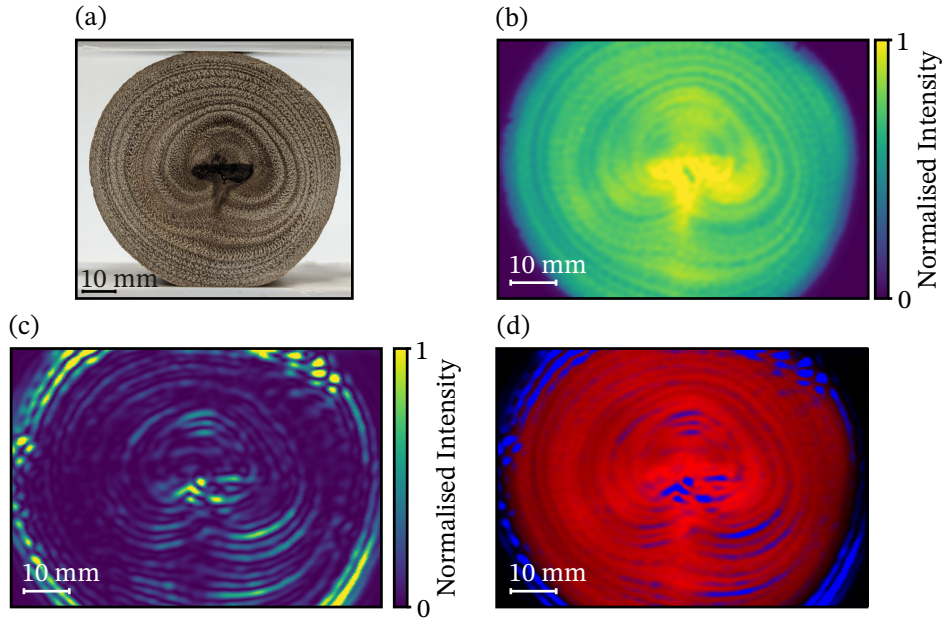
Figure 3.5: Detection of growth rings in cut Eucalyptus cladocalyx branch. (a) Photograph of the tree branch cross section. (b) Bright-field time domain image. (c) dark-field time domain image. (d) Composite image of bright and dark-field images mapped to red and blue colour channels respectively. We clip both images to the central 95% intensity distribution of data and map the intensity to the alpha channel of red and blue colour mattes, overlaying the dark-field onto the bright-field to form the composite.
