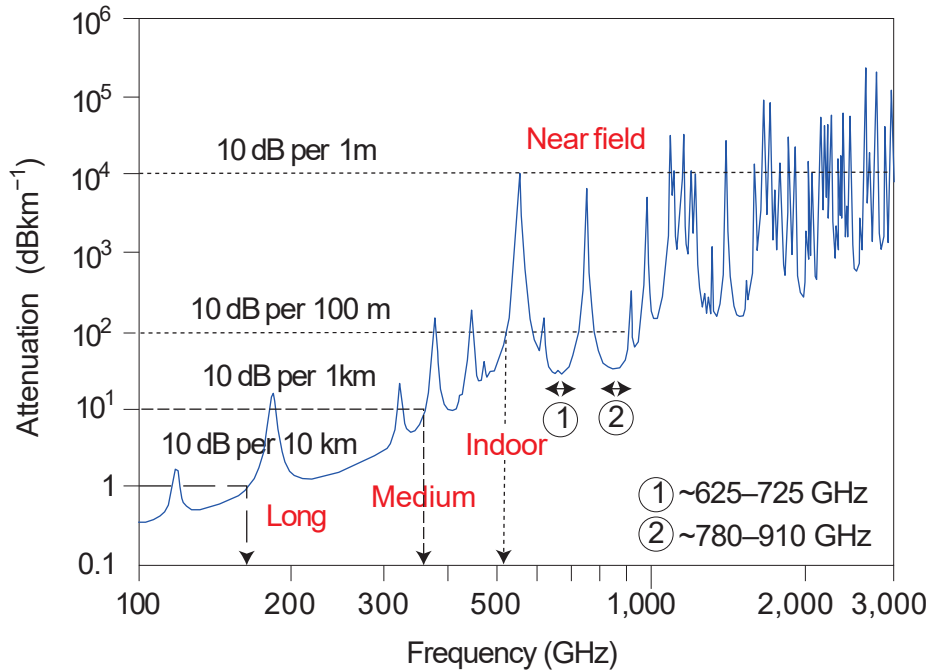
Figure 1.9: Transmission distance is limited by the attenuation, and the appropriate carrier frequency or frequency band is chosen by application, for example, long-distance, medium-distance, indoor and near-field communications. Above 600 GHz, there are two windows for indoor communications: ~625–725 GHz and ~780–910 GHz. Reprinted, with permission, from [61], with permission from Springer Nature.
