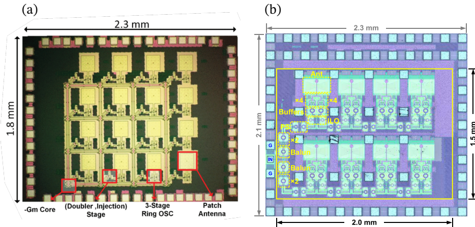
Figure 1.13: Examples of terahertz phased arrays. (a) 4 \times 4 phased array at 416 GHz. Adapted, with permission, from [121] © 2022 IEEE. (b) 4 \times 2 phased array at 298–334 GHz. Adapted, with permission, from [122] © 2025 IEEE.
