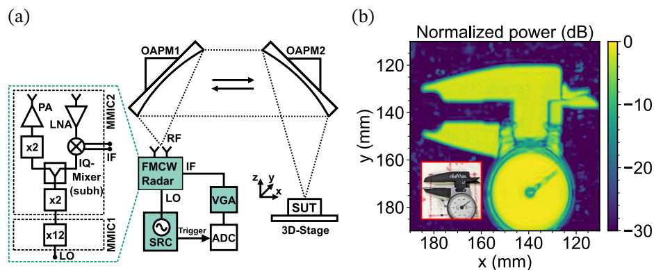
Figure 1.6: Example of high-resolution terahertz radar. (a) System block diagram, showing off-axis parabolic mirror focusing system. (b) terahertz image of the sample under test, a pair of callipers. Reproduced from Benjamin Baumann et al. [47]. Licensed under CC BY 4.0.
