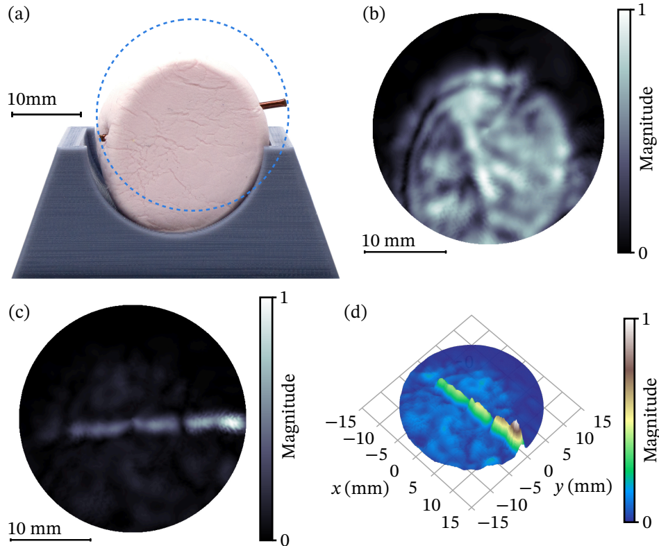
Figure 2.9: Demonstration of a food-safety application of terahertz imaging, namely the detection of a hidden wire inside a marshmallow. (a) Front view photo of the marshmallow with copper wire in 3D printed holder. (b) Observation plane at the front face of the marshmallow. (c) Weak reflection from the copper wire. (d) Contour plot differentiating the wire and the marshmallow.
