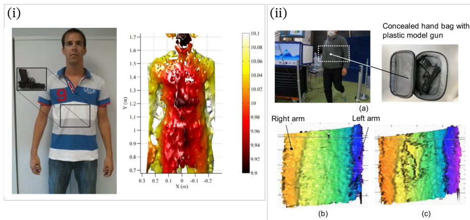
Figure 1.7: Examples of terahertz security screening applications. (i) Stationary terahertz FMCW radar at 300 GHz, revealing hidden replica gun. Adapted from [51] © 2015 IEEE. (ii) Walk-through terahertz FMCW radar at 290 GHz, revealing hidden replica gun. Reproduced from Ikari et al., [52]. Licensed under CC BY 4.0.
