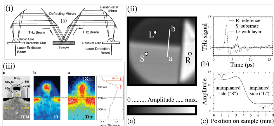
Figure 1.2: Examples of terahertz material characterisation applications. (i) Reflection based terahertz TDS setup for characterisation of doped semiconductors. Reprinted from [10], with the permission of AIP Publishing. (ii) Observation of terahertz TDS transmission affected by ion implantation on silicon sample. Reprinted from [12], with the permission of AIP Publishing. (iii) Comparison between transmission electron microscopy, infrared, and terahertz imaging for dopant regions in transistors. Reprinted with permission from [11]. Copyright 2008 American Chemical Society.
