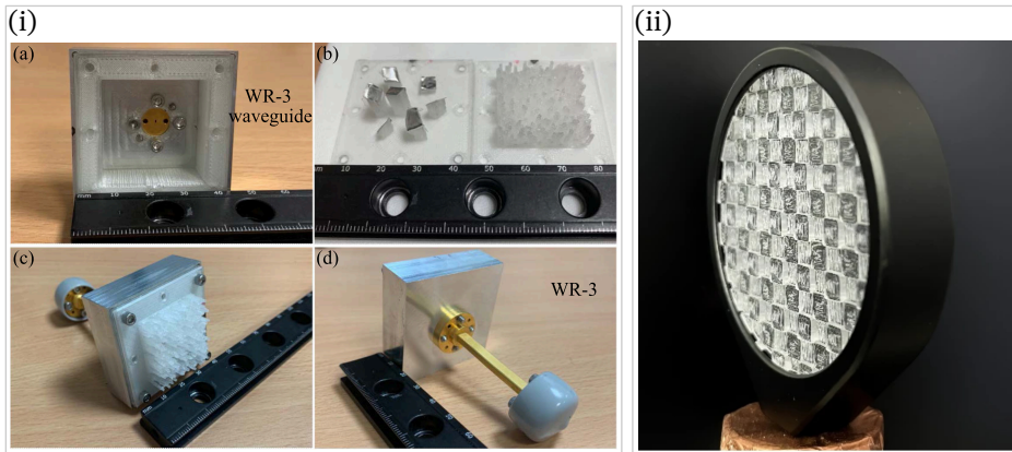
Figure 1.16: Examples of 3D-printed COC components. (a) 3D-printed COC cavity antenna for direction of arrival applications. Reprinted, with permission, from [148] © 2024 IEEE. (b) 3D-printed COC frequency reference. Reproduced from Tobias Kubiczek et al. [144]. Licensed under CC BY 4.0.
