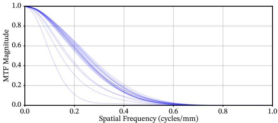
Figure 2.12: Monte Carlo tolerance analysis of the Risley-prism system in Ansys Zemax OpticStudio. Performed with a 0.2 mm tolerance for surface geometry and optic position. These results are comparable to those shown in Fig. 2.8(g).
