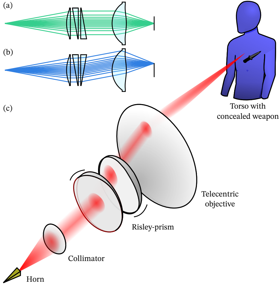
Figure 2.1: Conceptual model of a large scale terahertz imaging system using a Risley-prism and telecentric objective to detect concealed objects on a torso. (a) Minimum deflection and (b) maximum deflection configurations. (c) 3D illustration of the system, showing normal wave incidence on the target to maximize detectable power in reflection.
