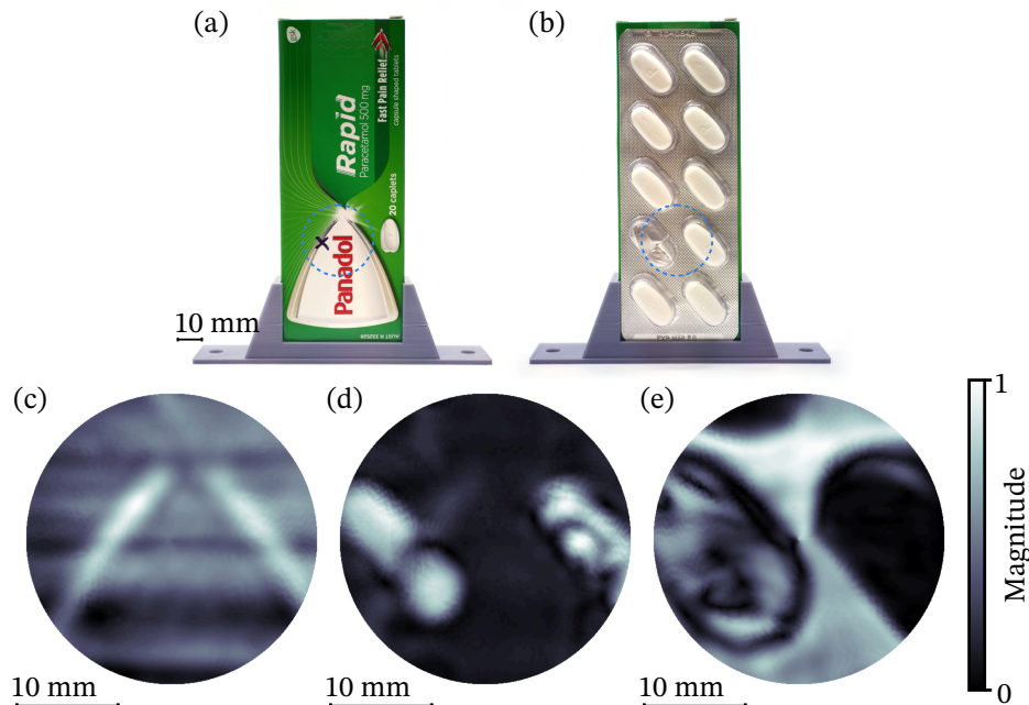
Figure 2.11: Demonstration of hidden and missing object detection. A tablet missing from a blister packet is revealed with terahertz imaging. (a) Front view photo. (b) Front view photo of blister packet outside of cardboard box to show the location of the missing tablet. (c) Observation plane showing small reflections from the metallic foil on the packaging. (d) Observation plane showing the top of the pre-formed plastic packaging. (e) Observation plane corresponding to the metallic backing of the blister packet. The stronger reflection on the left-hand side of the image indicates the missing tablet.
