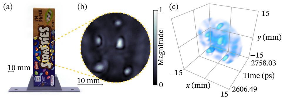
Figure 2.10: Demonstration of hidden object detection. Chocolates concealed inside a cardboard box are revealed with terahertz imaging. (a) Front view photo. (b) Observation plane showing the location of chocolates in the focal plane. (c) Volumetric render of dataset showing the locations of the chocolates in 3D space.
