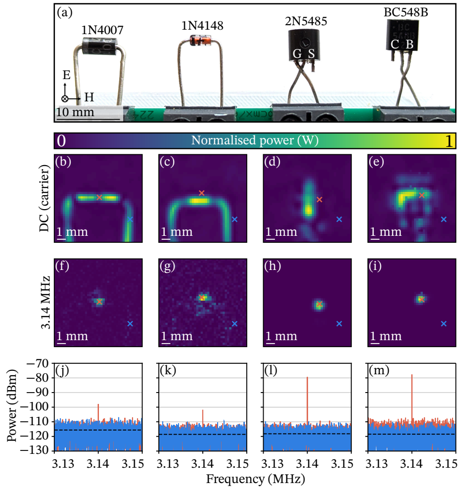
Figure 4.5: Localization of PN junctions in semiconductor components. (a) Photograph of 1N4007, 1N4148, 2N5485, and BC548B (left to right). The legs of the two rightmost devices are twisted for correct polarity. (b–e) Frequency domain raster-scans at 275 GHz. (f–i) Frequency domain raster-scans at 3.14 MHz offset frequency from the 275 GHz carrier. (j–m) Spectra of the four components, corresponding to the marked positions in the raster-scans. The pixels marked in red are the highest power pixels in the 3.14 MHz images, corresponding to the semiconductor region responsible for the sideband modulation, and those marked in blue are reference pixels. The black dashed lines indicates the mean of the spectra at the reference pixel and serve as the noise floor for SNR calculations [245]. The peak power spots in (b–e) differ from those marked in (f–i) due to the stronger reflection at the carrier frequency, which reveals internal metallic structures.
