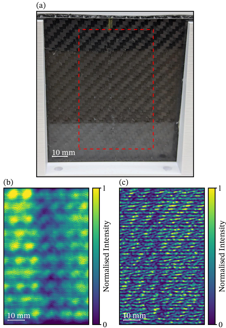
Figure 3.8: Defect detection on carbon fibre panel which has undergone a three-point bend test. (a) Photograph of the panel, with the vertical fracture approximately in the centre. (b) Bright-field time domain image. (c) Dark-field time domain image. We clip both images to the central 98% intensity distribution of data to remove any outliers.
