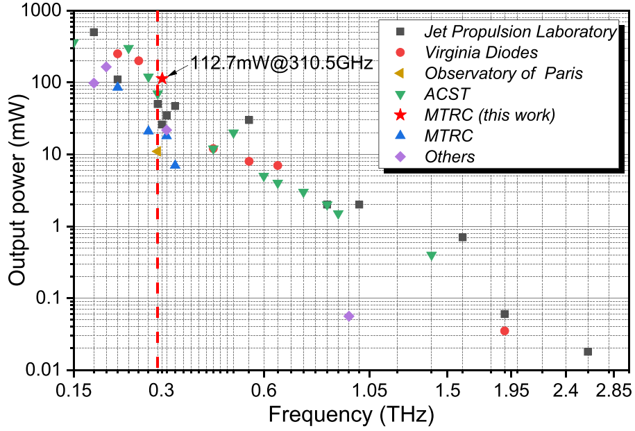
Figure 1.11: State-of-the-art frequency multiplied sources based on Schottky diode. Data table: Jet Propulsion Laboratory [72], [73], [74], [75], [70], [76], [77], Virginia Diodes [78], [79], [80], Observatory of Paris [81], ACST [82], [83], [84], [85], MTRC [86], [87], [88], [89], [90], Others [91], [92], [93], [94]. Reprinted, with permission, from [71] © 2025 IEEE
