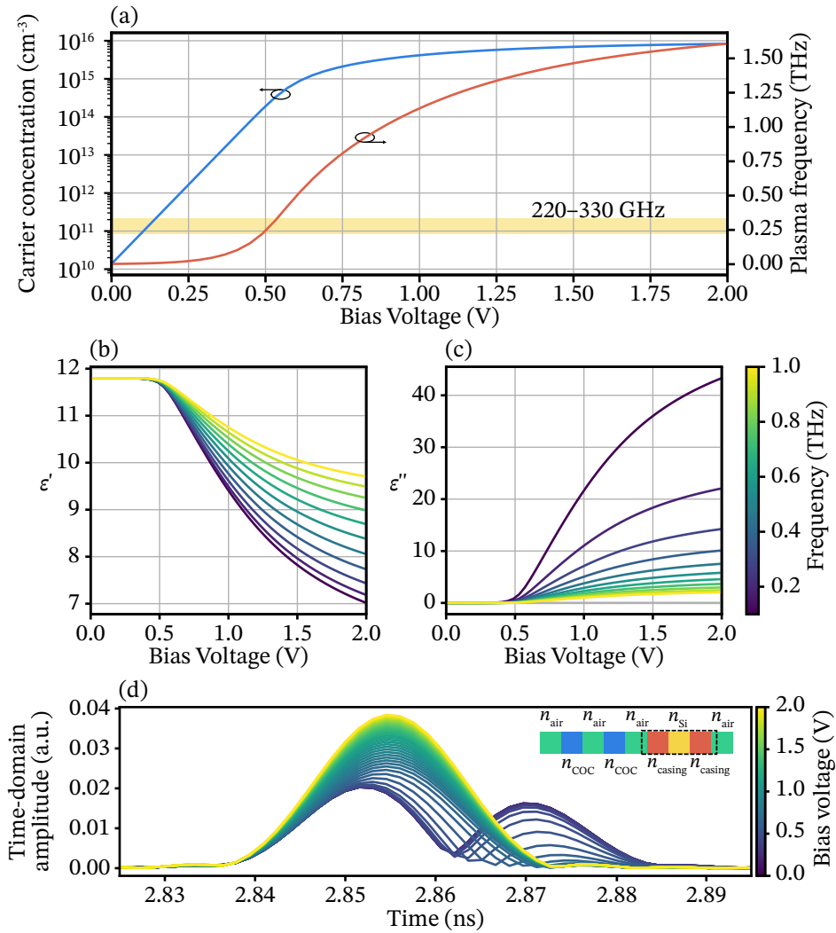
Figure 4.1: Simulation of terahertz interaction with free carriers in the PN junction. (a) Simulated electron and hole concentration over bias voltage steps, equal at the centre of the depletion region, and the resultant calculated electron plasma frequency. (b) Real and (c) imaginary components of the permittivity at the centre of the depletion region. (d) Absolute amplitude of calculated terahertz time-domain signals with a bandwidth between 220 and 330 GHz upon reflection from a packaged PN junction over bias steps of 0–2 V DC , with the peaks corresponding to the reflections from the air, diode casing, and silicon interfaces. The inset shows the configuration used for the Fresnel model calculations, where refractive indexes n_{\text{air}}=1 , n_{\text{COC}}=1.53 , and n_{\text{casing}}=1.5 , and the distances used to construct the model are [210, 15, 80, 43.546, 47.9, 0.25, 0.5, 0.25, 100] mm.
