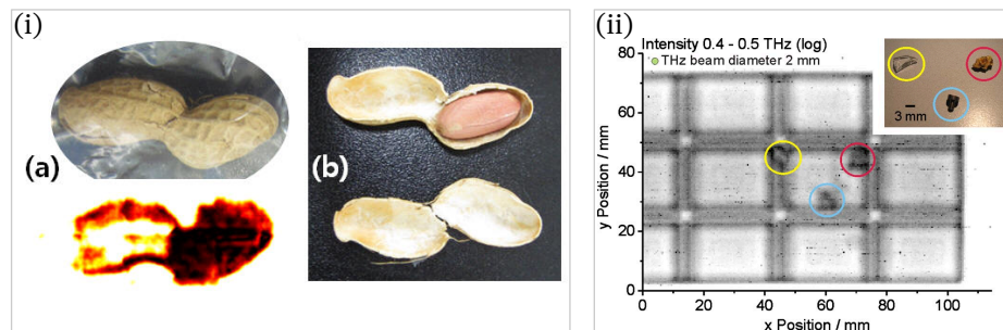
Figure 1.4: Examples of terahertz food inspection. (i) Demonstration of peanut imaging with terahertz gyrotron. Reprinted, with permission, from [36] © 2012 IEEE. (ii) Demonstration of terahertz imaging to detect glass, stone, and metal contaminants in a chocolate bar. Used with permission of Jördens et al., from [37]; permission conveyed through Copyright Clearance Center, Inc.
