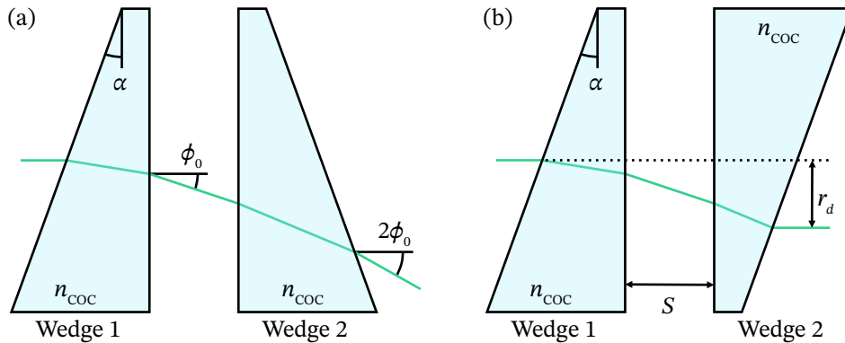
Figure 2.2: Ray trace diagram of an incident normal beam through a Risley-prism. Both wedges feature an inline angle \alpha . (a) Maximum deflection configuration. (b) Minimum deflection configuration showing the centre offset r_d .
