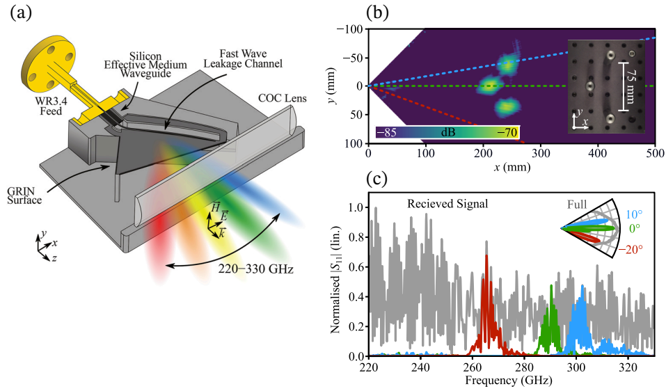
Figure 1.12: Leaky-wave antenna illustration and experiment. (a) Illustration of leaky-wave antenna and packaging with cyclic olefin copolymer (COC) lens. (b) Experimental demonstration of simultaneous target tracking. (c) showing frequency mapping of direction. Adapted from Harrison Lees et al. [118]. Licensed under CC BY.
