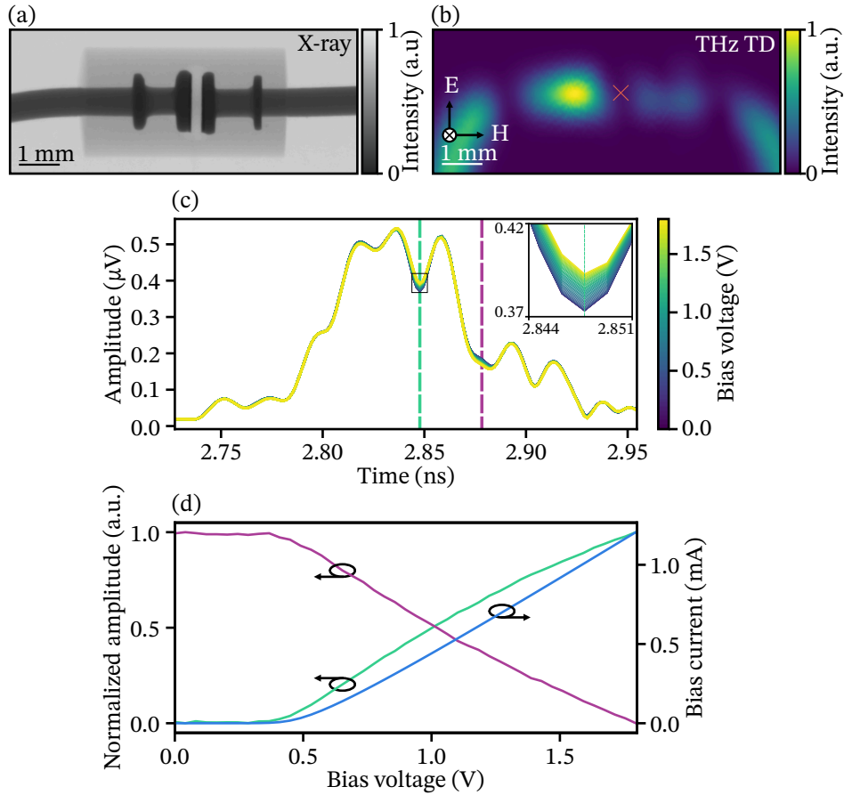
Figure 4.4: Bias voltage ramping at low frequency showing the change in the reflected time-domain signal. (a) X-ray image of the 1N4007 diode. (b) Terahertz time-domain raster image of the diode, obtained with VNA configuration. The wire leads are bent downwards for mounting. The red cross indicates the location of the focal spot for the measurement. (c) Time-domain trace of the central pixel corresponding to the PN junction of the diode, obtained with the IQ configuration. The inset highlights the change in reflectivity from the PN junction. The time, i.e., depth, axis is perpendicular to the plane of (a) and (b). (d) Voltage-dependent amplitude of (c) at the time-domain points indicated by the dashed lines, corresponding to the front and back of the PN junction.
