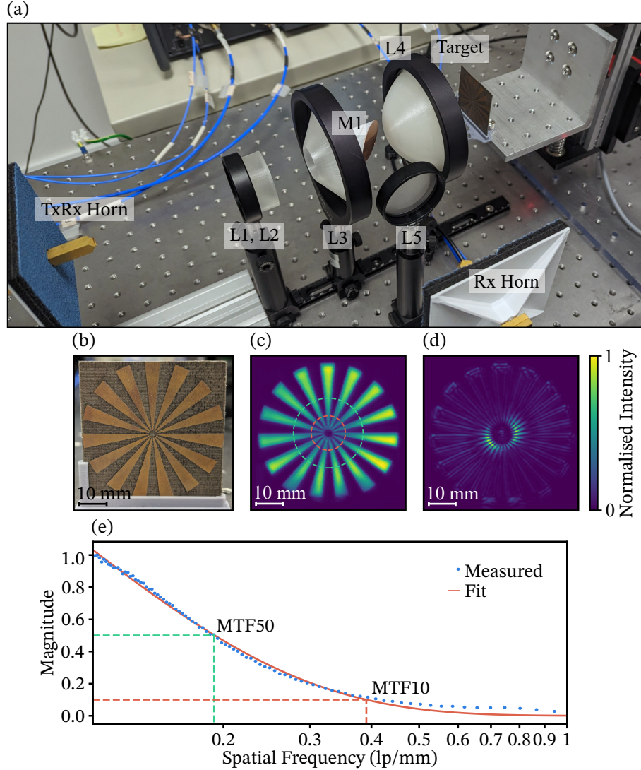
Figure 3.3: Spatial resolution test of the imaging system. (a) Photograph of the experimental imaging system with the resolution test target positioned at the focal plane of the objective. L1: Horn collimating lens; L2: Diverging axicon lens; L3: Collimating axicon lens; L4: Objective lens; M1: 45° mirror; L5: Collector collimating lens. (b) Photograph of the resolution test target. (c) Bright-field time domain image. (d) Dark-field time domain image. (e) Modulation transfer function of the bright-field scan, indicating a MTF10 of 0.391 lp/mm and MTF50 of 0.192 lp/mm.
