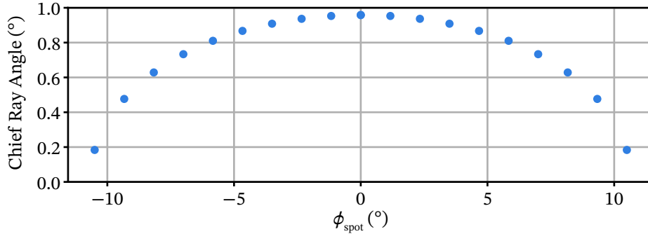
Figure 2.5: Chief ray angle over \phi_{\text{spot}} , along the x -axis of the image plane. Computed with the Risley-prism in conjunction with the telecentric objective, at various configurations, like those shown in Fig. 2.1(a,b).
