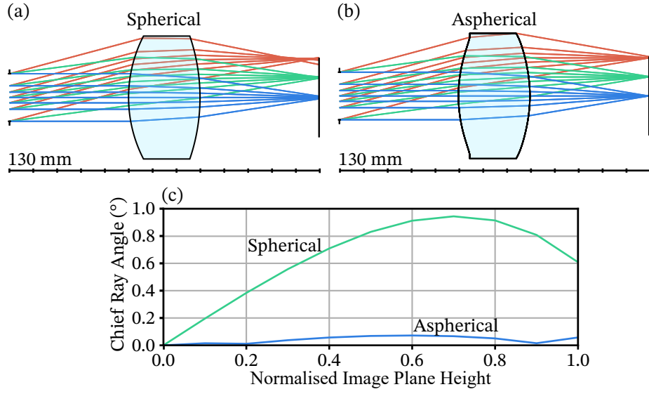
Figure 2.4: Simplified comparison between spherical and aspherical surfaces for telecentric lens design. Both lenses are optimized with the same figure of merit to minimize spot size and chief ray angle, from a beam diameter of 20 mm with up to 15° deflection. (a) Spherical biconvex lens, showing aberrations at maximum field angle. (b) Aspheric biconvex lens, with reduced aberrations compared to the spherical design. (c) Chief ray angle over the image plane. For optimization, the distance from the entrance pupil to the first surface and the distance from the second surface to the image plane are fixed at 50 mm. The thickness of the lens is fixed at 30 mm. The radii of the spherical surfaces are variable. The radii, conic constant, and even-aspheric coefficients of the aspheric surfaces are variable.
