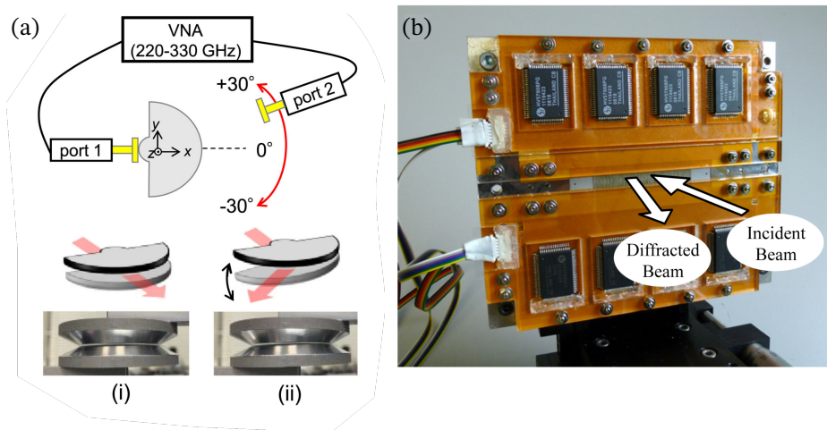
Figure 1.14: Examples of terahertz reconfigurable optics. (a) Mechanically adjustable Luneburg lens. Reprinted, with permission, from [126] © 2020 IEEE. (b) Reconfigurable diffraction grating. Reproduced from Y. Monnai et al. [128]. Published by Optica Publishing Group under the terms of the OSA Open Access Publishing Agreement.
