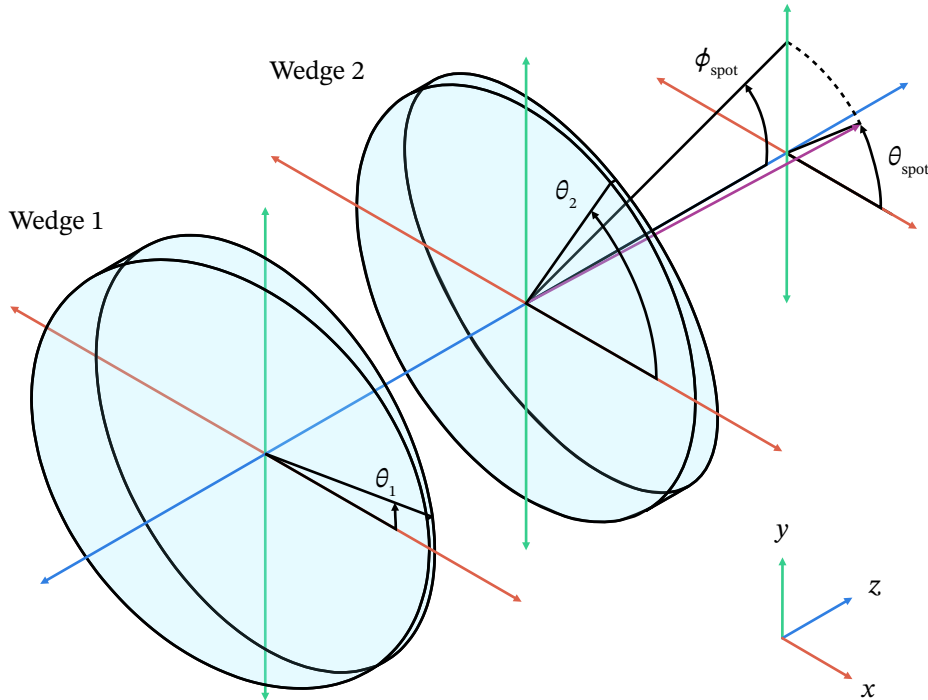
Figure 2.3: Illustration of the Risley-prism coordinate space. Each wedge is rotated about the z -axis by angle \theta_k , where k is the wedge number. \theta_1 and \theta_2 for a desired \phi_{\text{spot}} and \theta_{\text{spot}} are found using the two step inverse method [181].
