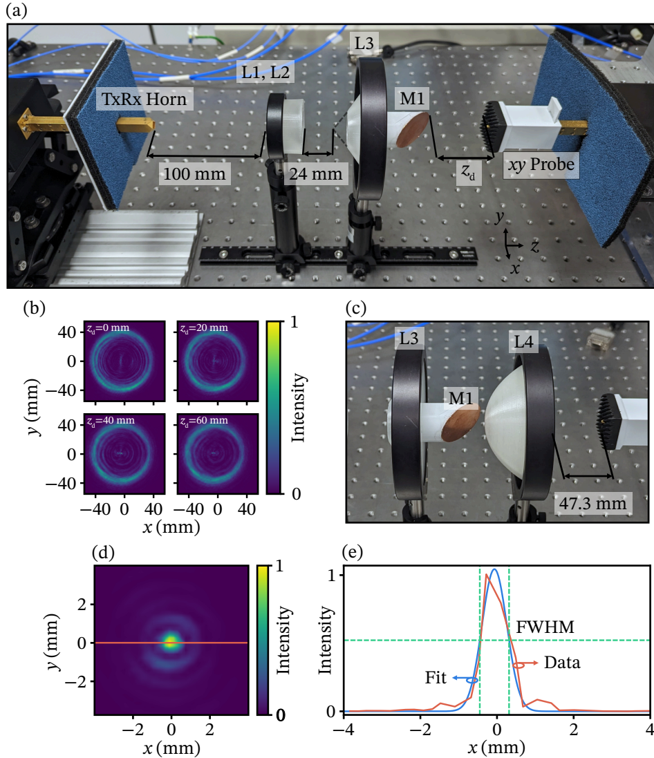
Figure 3.2: Near field scanning setup of the imaging system. (a) Photograph of scanning setup to observe the collimated annular-beam. L1: Horn collimating lens; L2: Diverging axicon lens; L3: Collimating axicon lens; M1: 45° mirror. The dark-field collector components are not included here. (b) Transmission raster scans along of the xy plane at z = 0 –60 mm, showing the collimated ring at 275 GHz. (c) Photograph of the objective lens, L4, positioned after the second axicon, L3, with scanning setup to measure the spot size. (d) Transmission raster scan along the xy plane showing the location of the system focus at 275 GHz, cropped to \pm 4 mm. (e) Cross section at y = 0 , showing a FWHM of 0.763 mm, calculated from the fitted Gaussian curve.
