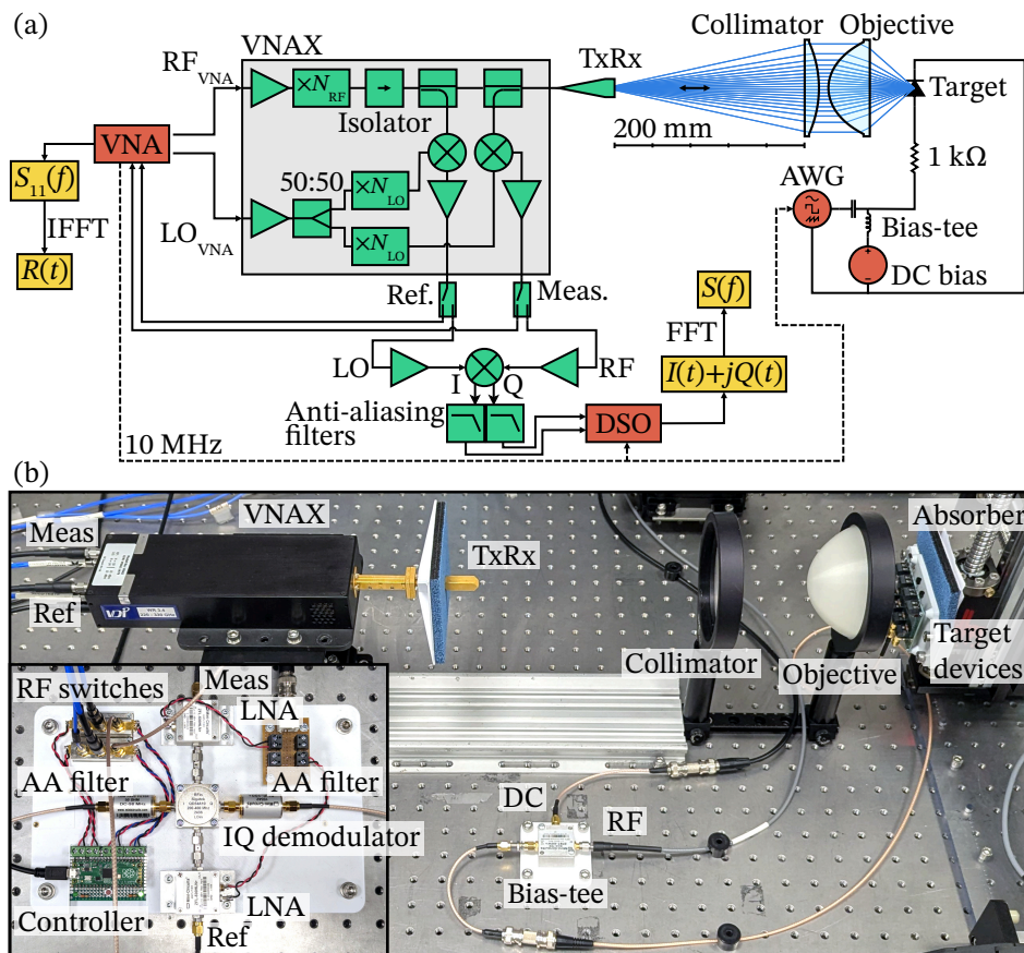
Figure 4.3: Integrated quadrature receiver system. (a) Diagram of the experimental setup used to measure complex reflection over 220–330 GHz. A vector network analyzer (VNA) extension module (VNAX) [231] is used to down-convert the terahertz carrier to an intermediate frequency, providing a reference (Ref.) of the transmitted signal, and a measurement (Meas.) signal encoded with the modulation from the target. RF switches are used to switch data acquisition between the VNA and the custom IQ demodulator attached to the digital storage oscilloscope (DSO) for digital signal processing; the VNA configuration is used for imaging, and the DSO configuration is used for observing carrier sidebands and temporal measurements. The VNA provides the 10 MHz reference clock for the DSO and the AWG (used for megahertz frequency bias). (b) Annotated photograph of the setup. The inset shows the IQ demodulator with LO and RF low noise amplifiers (LNA), and the anti-aliasing filters for the I and Q signals. 3D printed cyclic olefin copolymer lenses collimate and focus the beam from the horn antenna to an approximately 1.3-mm spot on the diode. The diode is retained in a screw terminal block and held 47.3 mm away from the objective lens.
