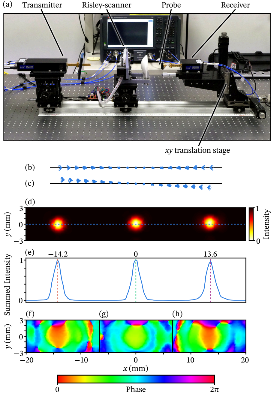
Figure 2.7: Calibration of the system scanning region. A S_{21} raster-scan is taken for each azimuth position of -10.5^\circ , 0^\circ , 10.5^\circ with a near-field probe. (a) Side view photo of the raster scanning setup. (b) Ray-traced footprint diagram showing the spot positions along the x-axis; see Visualization 1. (c) Footprint diagram showing the effect of wedge positioning error. With both wedges offset -3^\circ , there is rotation along the points. (d) Three raster scans of S_{21} intensity at 275 GHz normalized and summed, with probe at the focal plane. (e) Cross section at the midpoint of the summed intensity scans showing 27.8 mm between the two furthest points. (f–h) Phase profile of each raster scan at 275 GHz.
