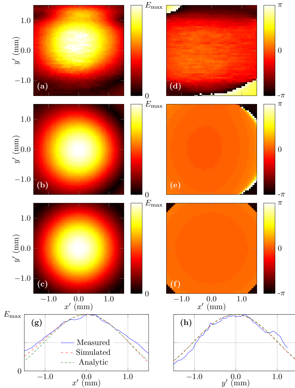
Figure 7.7. Measured focal spot of DRA-based reflectarray. Beam profile of focal spot at 1 THz. (a) Measured field magnitude distribution, (b) simulated field distribution, (c) analytically predicted field distribution (Horváth and Bor 2003), (d,e,f) corresponding phase profiles for (a,b,c) respectively, and (g,h) cross-sectional linear field distribution amplitudes. Note the measured profile in (h) is offset to coincide with the other plots. All plots are in linear scale. After Headland et al. (2016a).
