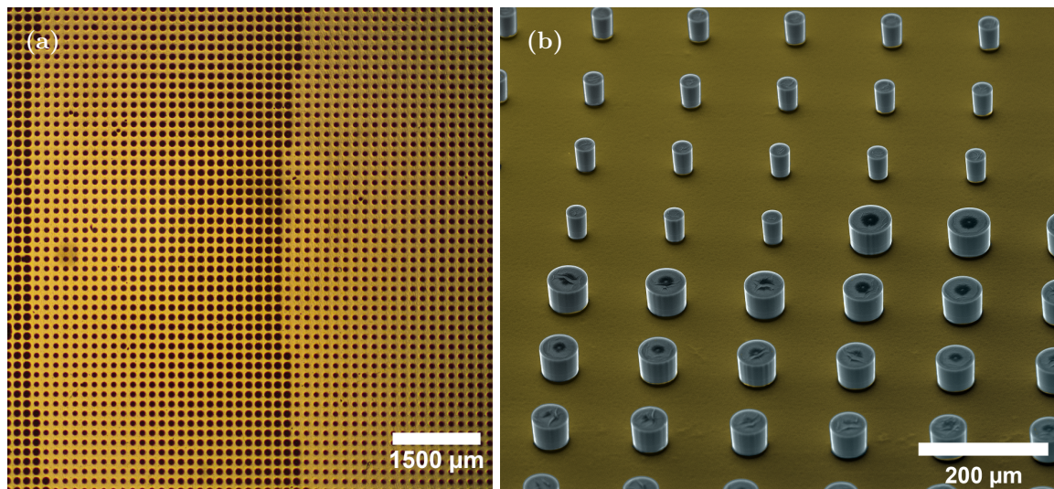
Figure 7.5. Fabricated terahertz reflectarray design. Realised reflectarray structure, showing (a) optical microscope image, and (b) and false-colour scanning electron micrograph. After Headland et al. (2016a).
