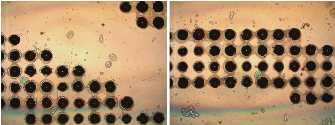
Figure 9.6. Hole lattice zone plate sample. Optical micrographs of back-side of fabricated hole lattice sample, showing incomplete etch, as evidenced by the apparent lack of holes in alternating zones.
