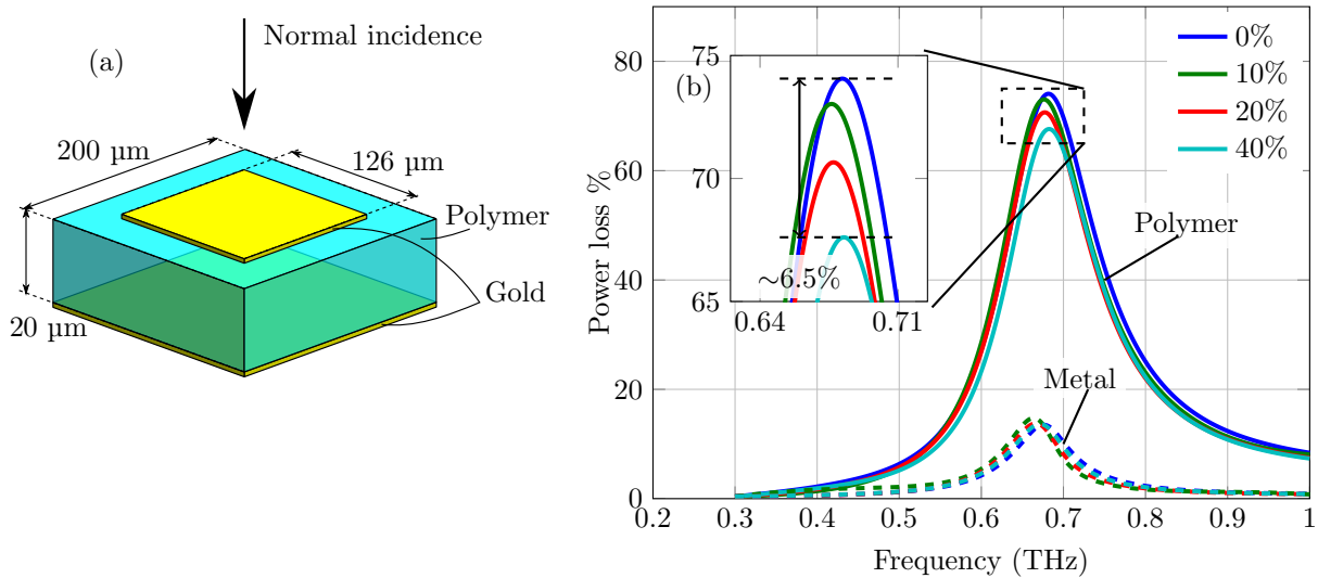
Figure 4.4. Doped PDMS-based resonator. Simulations to determine the impact of this new doped PDMS material on a hypothetical metallic resonator, showing (a) the structure of a unit cell of the resonator, showing incident excitation, where it is noted that the polymer in question is doped PDMS, and (b) a breakdown of the origins of loss in the metallic resonator, for the four different concentrations of PTFE tested, where dielectric loss is given with solid lines and Ohmic dissipation is represented with dashed lines.
