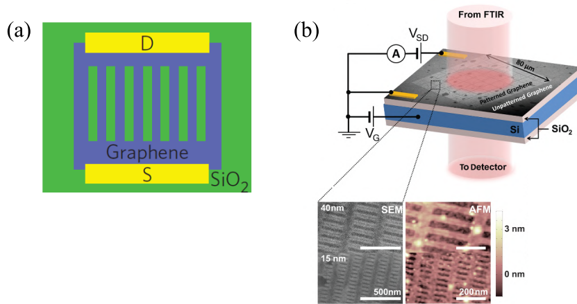
Figure 1.17. Electrically tunable terahertz metamaterials based on graphene plasmonics.
