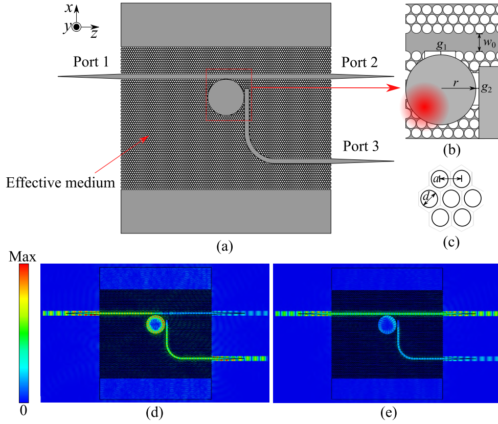
Figure 3.1. Terahertz 1-to-2 switch using an integrated disk resonator on substrateless dielectric waveguide platform. The waveguides with a width w_0 of 225 \mu\text{m} are built into a free-standing wafer with a thickness of 250 \mu\text{m} . (a) Top view, the unperforated silicon slab is for handling purposes, while the taper structures are for mode transition between the sample and the feeding hollow waveguides in measurements. The dimensions of the terahertz 1-to-2 switch are 10 mm in width and length. (b) Coupling region of disk resonator with a radius r of 863 \mu\text{m} and a separation from the waveguide g_1 and g_2 of 20 \mu\text{m} . The red dot is a pumping area of the red laser. (c) Hexagonal lattice of the effective medium cladding with perforation period a of 100 \mu\text{m} and an air hole diameter d of 90 \mu\text{m} . (d) and (e) Simulated instantaneous field distributions are plotted in linear scale at 275 GHz for the neutral and pumped switch resonator, respectively.
