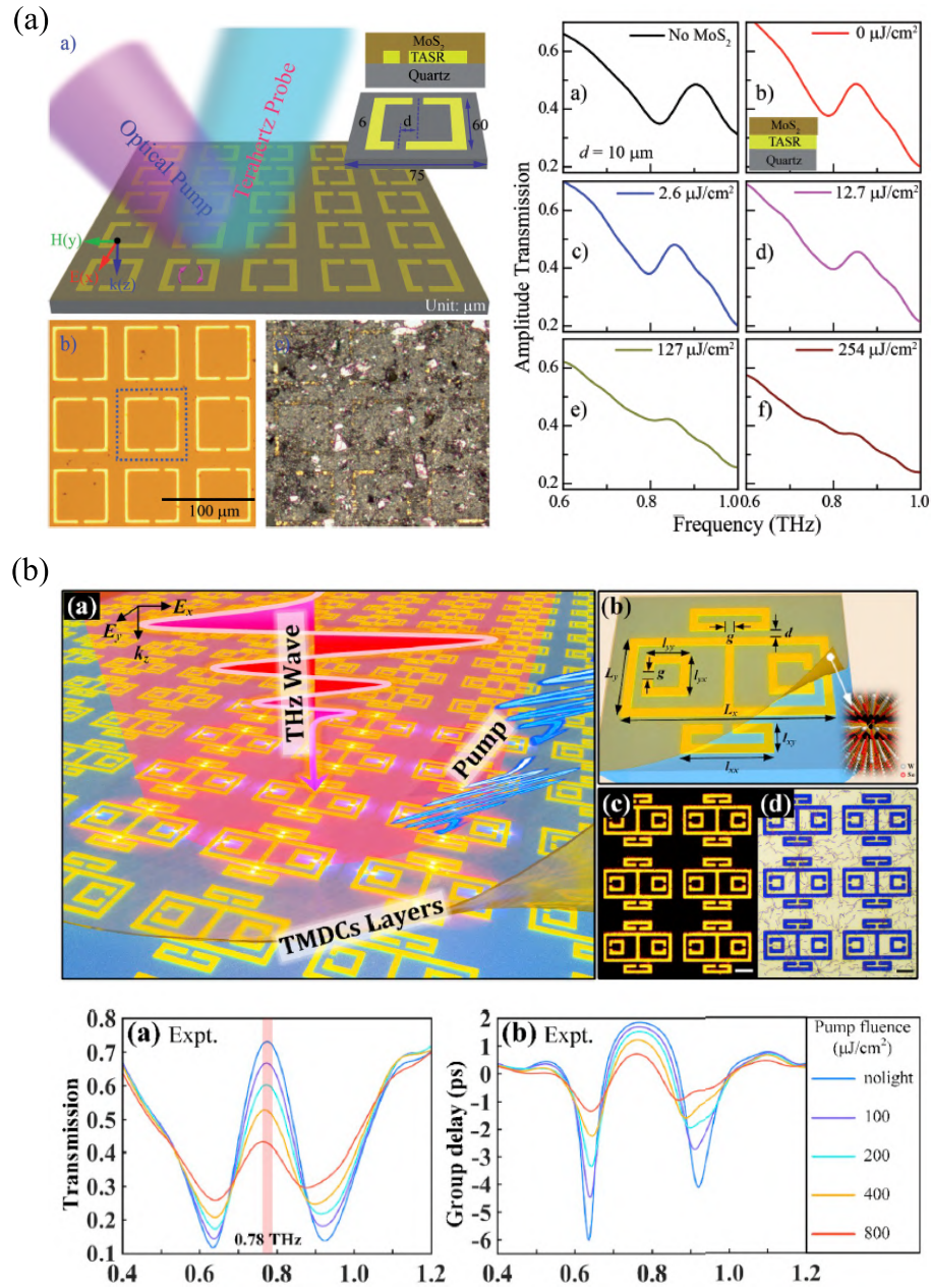
Figure 1.15. Optically tunable terahertz modulators based on 2D materials. (a) Ultrafast switching and modulation of the Fano resonances in MoS 2 -coated metamaterials. Adopted from Srivastava et al. (2017), and (b) ultrafast switching and amplitude modulation based on WSe 2 -functionalised metaphotonic devices. Adopted from Hu et al. (2020a).
