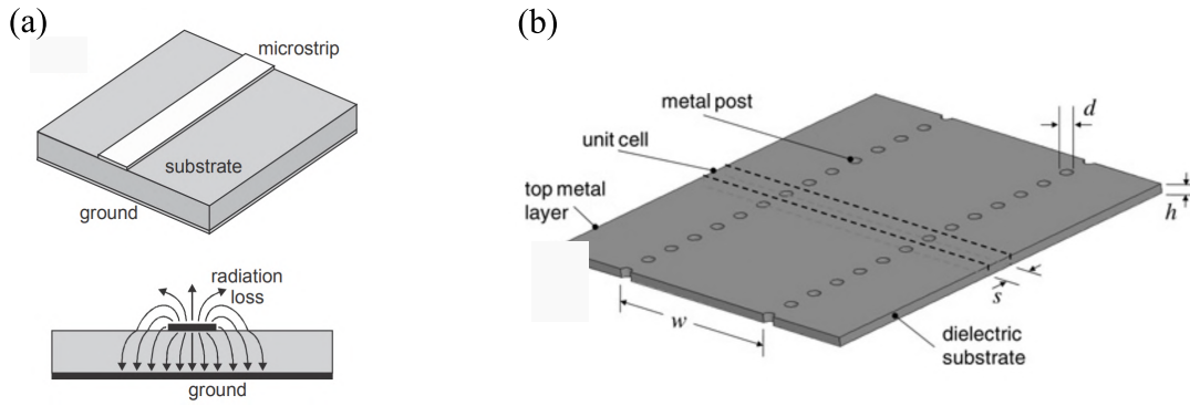
Figure 1.4. Microwave-inspired waveguides. (a) Microstrip lines. Adopted from Zakaria et al. (2010), and (b) Substrate-integrated waveguides (SIW). Adopted from Bozzi et al. (2011).
