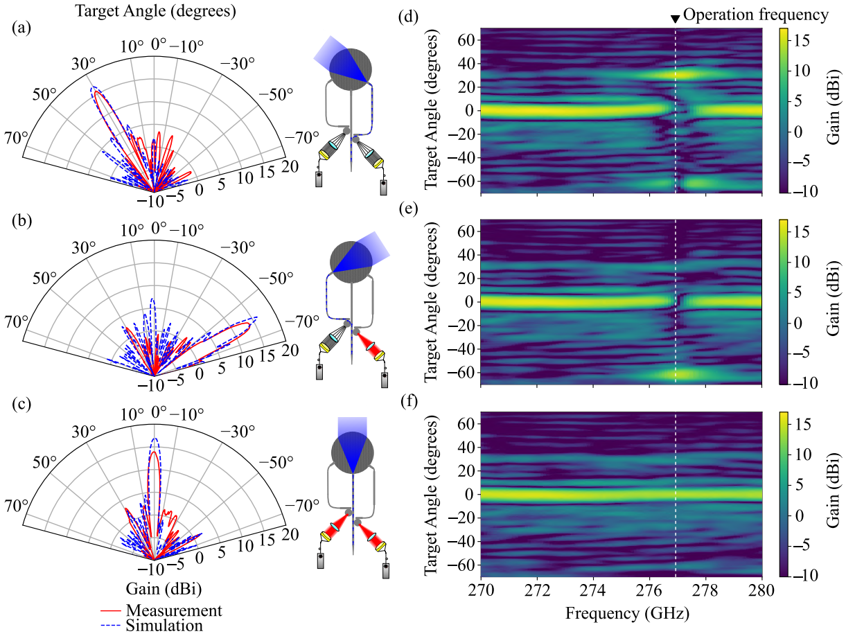
Figure 3.9. Simulated and measured radiation patterns of the three-port switched beam at 276.98 GHz. (a) Both Disks are in the neutral state for 30° output. (b) Disk 1 pumped for -60° output. (c) Both Disks are pumped for 0° output. (d)-(f) Measured radiation patterns of the three-port switched beam according to (a), (b), and (c), respectively.
