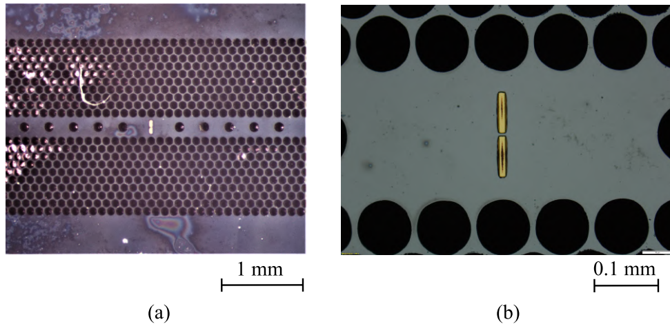
Figure 4.3. Fabricated modulator. (a) Terahertz modulator comprising of the dipole resonator and the photonic crystal cavity on the substrateless silicon platform. (b) Micrograph of the dipole resonator on the top of the waveguide core. The etched through holes of the platform are visible as white holes, while incomplete etching of 6 \mu\text{m} in device thickness results in the blind holes in (a).
