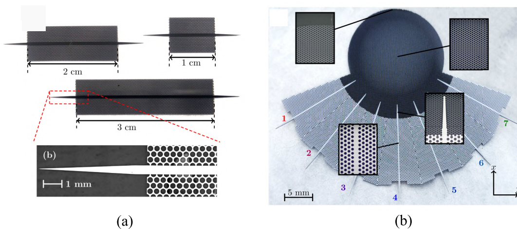
Figure 1.5. Terahertz photonic crystal waveguides and associated passive components.
