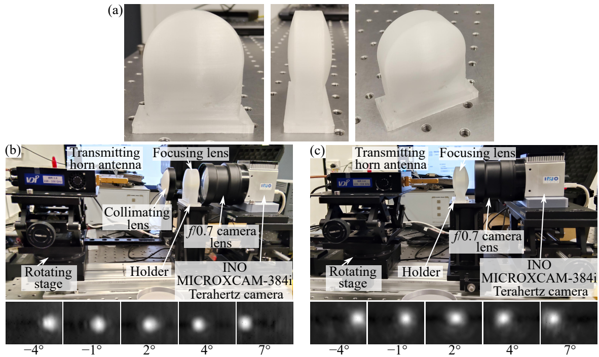
Figure 4.7. Lens design and characterisation. Design and experimental characterisation of the focusing lens. (a) 3D-printed aspheric bi-convex lens with integrated holder, including front, side, and perspective views. (b) Measurement setup and representative spatial focusing for the collimated input case using a collimating lens. (c) Measurement setup and representative spatial focusing for the divergent input case without a collimating lens. The measurement system consists of a WR-3.4 source, the fabricated lens, and an INO MICROXCAM-384i terahertz camera with an f/0.7 lens. The WR-3.4 source is fixed at 300 GHz and rotated to generate incident angles from -4^\circ to 7^\circ , emulating the angular beams expected from frequencies 280 GHz, 290 GHz, 300 GHz, 310 GHz, and 320 GHz, respectively. The resulting focal spots recorded by the INO MICROXCAM-384i terahertz camera are shown below each setup.
