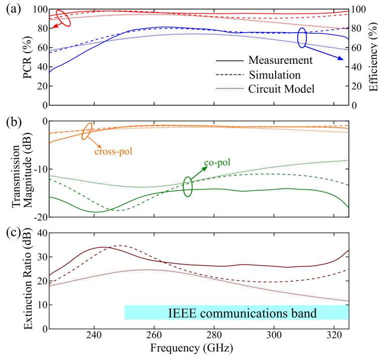
Figure 2.10. Half-wave plate performance. Performance parameters for the proposed device working as a half-wave plate at s = 150 \mu\text{m} . (a) PCR and efficiency, (b) co and cross-polarisation transmission magnitudes, and (c) extinction ratio.
