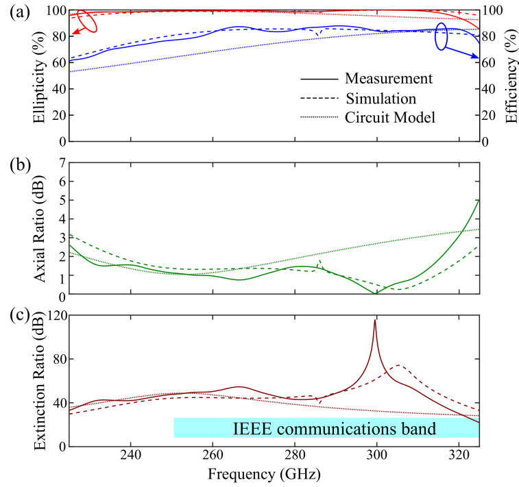
Figure 2.7. Quarter-wave plate performance. Performance parameters for the proposed device working as a quarter-wave plate at s = 0 \mu\text{m} . (a) Ellipticity and efficiency, (b) axial ratio, and (c) extinction ratio.
