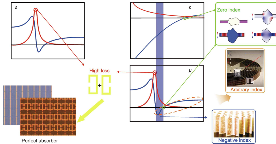
Figure 1.4. Examples of exceptional electromagnetic responses enabled by metamaterial unit cell design. Some widely implemented unit cell structures enabling various refractive index values achieved through metamaterial design, exhibiting exquisite phenomenon, such as negative indexes (Shelby et al. , 2001), zero-index materials (Mahmoud and Engheta, 2014), metamaterial perfect absorbers (Tao et al. , 2008), and the invisibility cloak (Schurig et al. , 2006). \epsilon : permittivity; \mu : permeability. Adopted from Sun and Zhou (2025).
