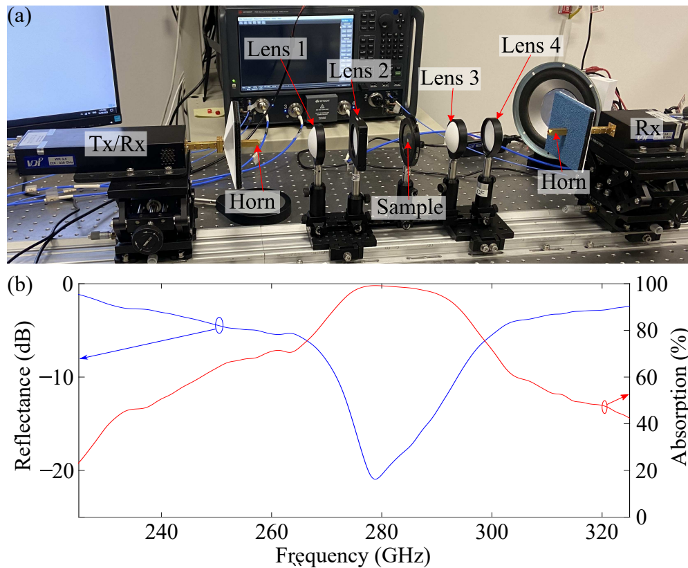
Figure 3.6. Electromagnetic measurement setup and response. Experimental setup and characterisation of terahertz response. (a) Measurement setup with four lenses and sample at the centre. (b) Measured electromagnetic response showing reflection and corresponding absorption across the 225–325 GHz range. Transmittance is below -100 dB and is therefore omitted for clarity.
