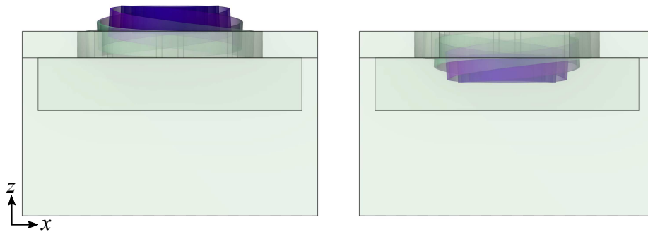
Figure 3.3. Simulated vibrational mode. COMSOL Multiphysics based simulated out-of-plane (up–down) vibrational mode of the niobium spiral structure at baseline mechanical resonance frequency of 12.20 kHz. Purple colour indicates the vertical displacement amplitude. The model includes the niobium spiral, COC substrate with an air gap, and the patterned gold reflector, accurately representing the full multilayer device geometry.
