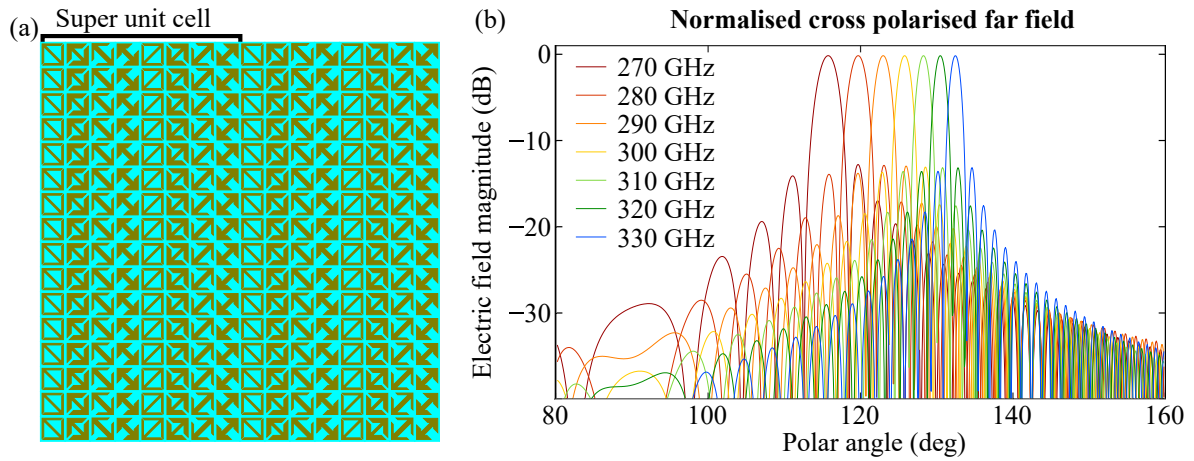
Figure 4.5. Metasurface design and response. Array-level implementation and response of phase-gradient beam deflection. (a) Metasurface design illustrating the arrangement of the middle resonant layer used to realise the phase gradient. Eight unit cells form a supercell covering the full 2\pi phase range. (b) Normalised cross-polarised far-field radiation patterns demonstrating frequency-dependent beam deflection across 270–330 GHz at 10 GHz intervals, with deflection angles of 116^\circ , 120^\circ , 123^\circ , 126^\circ , 128^\circ , 131^\circ , and 132^\circ with respect to the opposite normal.
