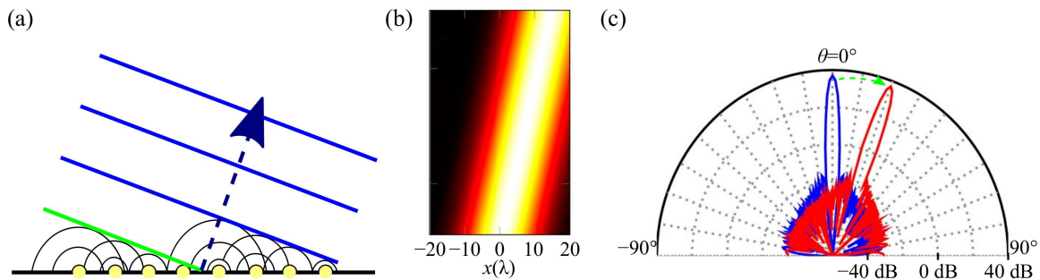
Figure 4.2. Phase gradient beam deflection. Illustration of angular beam deflection using phase control. (a) Huygens'-principle diagram for beam deflection. (b) Corresponding propagation beam deflection, and (c) far-field radiation pattern produced (red), showing a beam deflected from plane wave propagation (blue). Adopted from Headland et al. (2018).
