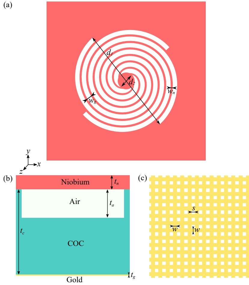
Figure 3.1. MEMS bolometer device layout. Schematic of the MEMS bolometer structure. (a) Top view showing the niobium Archimedean spiral antenna, with spiral diameter d_1 = 360 \mu\text{m} , core diameter d_2 = 60 \mu\text{m} , spiral arm width w_n = 7 \mu\text{m} , gap between spiral arms w_g = 15 \mu\text{m} . (b) Cross-sectional schematic illustrating the layered structure comprising a niobium absorber with thickness t_n = 50 \mu\text{m} , air cavity with thickness t_a = 100 \mu\text{m} , cyclic olefin copolymer (COC) support with thickness t_c = 300 \mu\text{m} , and gold back reflector with thickness t_g = 1 \mu\text{m} . (c) Patterned gold backplane showing periodic square apertures with gold strips of width w = 20 \mu\text{m} and spacing s = 20 \mu\text{m} .
