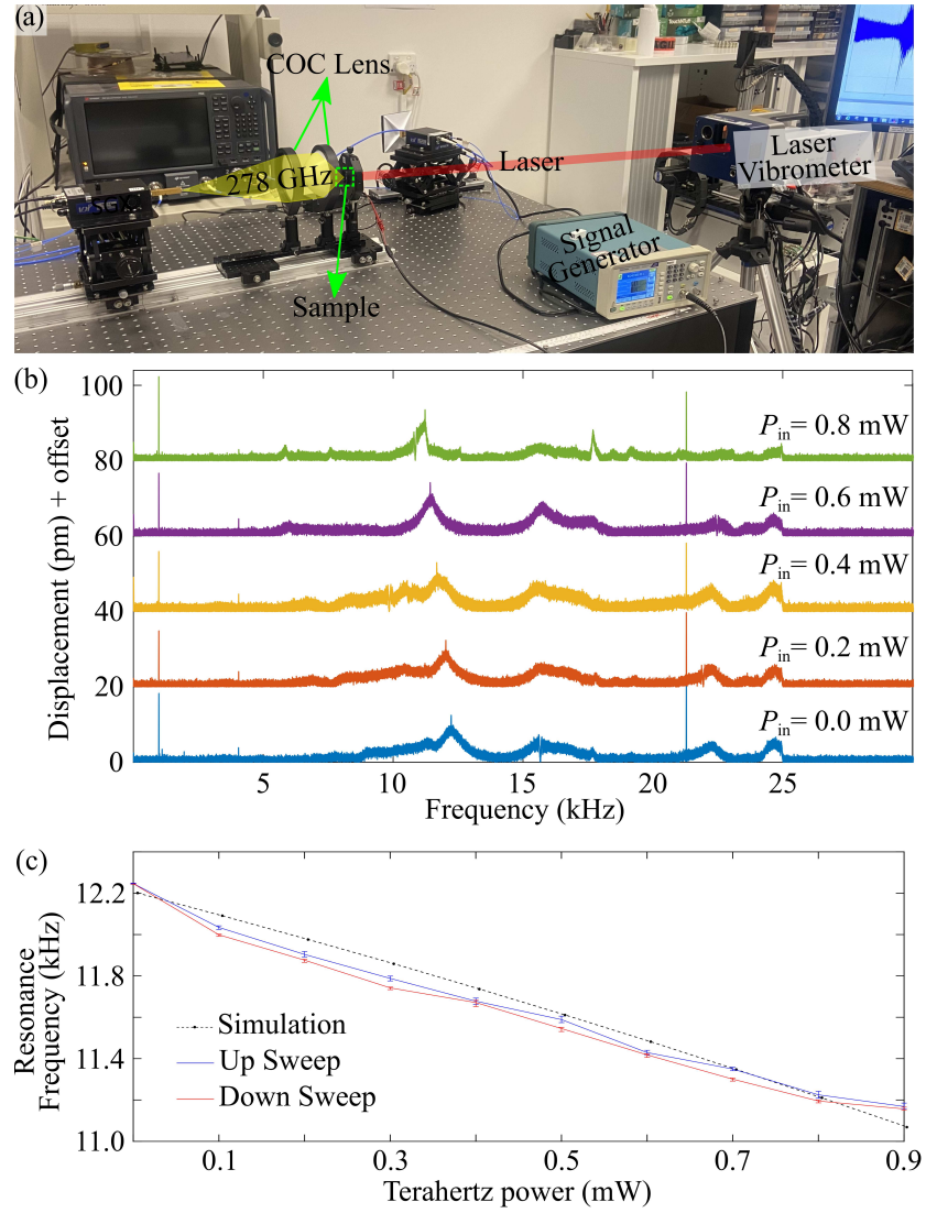
Figure 3.7. Mechanical measurement setup and response. Experimental setup for characterisation of the mechanical response. (a) Measurement setup with a continuous terahertz wave at 278 GHz incident from the SGX to the niobium spiral. On the opposite side, a laser beam from the LDV is incident to the spiral through the patterned gold and COC. Signal generator is connected to the piezoelectric chip to excite mechanical resonance. (b) Measured out-of-plane displacement spectra of the niobium spiral bolometer under increasing terahertz power levels (0 to 0.8 mW), acquired using laser Doppler vibrometry. Each curve is vertically offset for visual clarity. No vibrational response is observed beyond 25 kHz due to the 1–25 kHz range of the piezoelectric chip excitation. (c) Simulated and measured resonance frequency as a function of incident terahertz power, showing both measured up-sweep and measured down-sweep trends. Each measured point has error bars from five separate readings.
