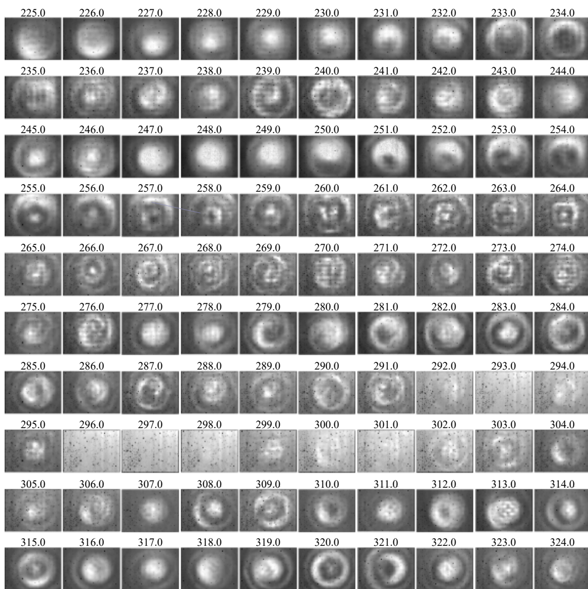
Figure B.1. Terahertz camera calibration. Raw intensity images captured using the WR-3.4 source and the terahertz camera equipped with an f/0.7 lens, without the metasurface, to characterise the native response of the detection system.
