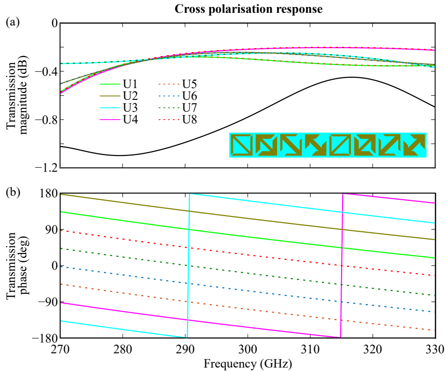
Figure 4.4. Unit cell transmission. Cross-polarised transmission of the eight individual elements. (a) Magnitude, and (b) phase. The labels U1–U8 refer to the unit cells illustrated in Figure 4.3(e). Unit cells with identical transmission magnitudes share the same geometrical parameters and are mirror symmetric about the vertical axis, resulting in a 180^\circ transmission phase shift. The black solid curve in (a) shows the simulated first-order cross-polarised transmission magnitude of the super unit cell formed by arranging the eight elements horizontally to provide a full 2\pi phase coverage. The inset in (a) illustrates the arrangement of the eight unit cells within the super unit cell.
