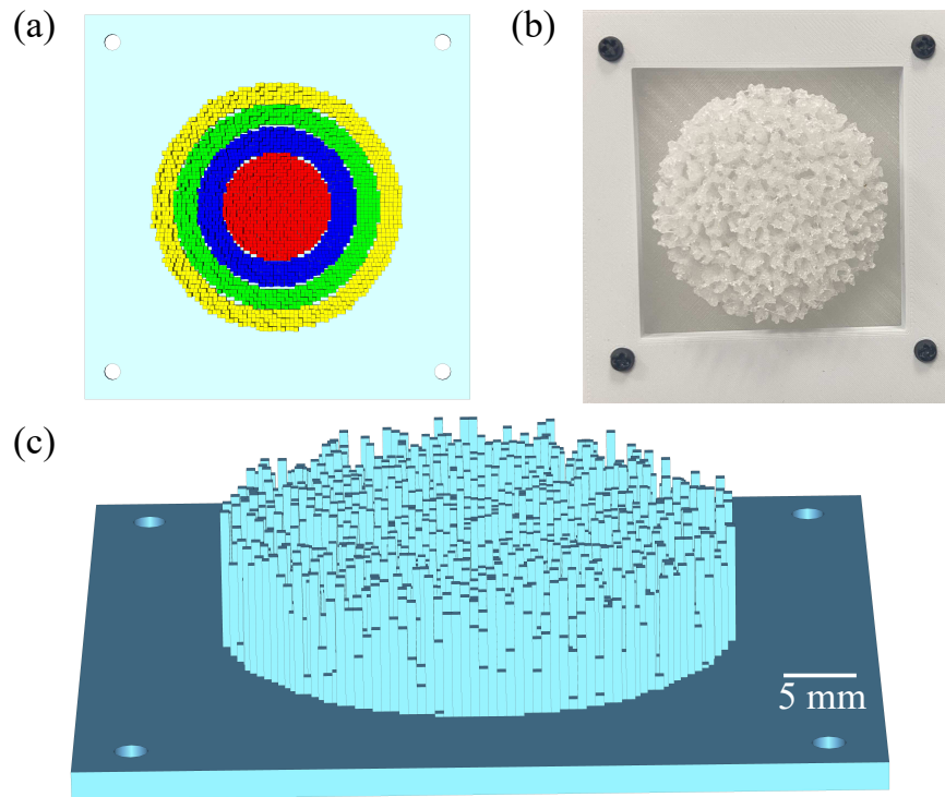
Figure 5.1. Design of the pseudo-random metasurface. 3D-printed pseudo-random metasurface, designed on a square platform with four screw holes for mounting onto the holder. (a) Top view CAD rendering highlighting four concentric zones with square pillars of widths 487\ \mu\text{m} (red), 524\ \mu\text{m} (blue), 568\ \mu\text{m} (green), and 619\ \mu\text{m} (yellow). Each zone contains 800 pillars with zone radius of 8.1\ \text{mm} (red), 11.9\ \text{mm} (blue), 15.2\ \text{mm} (green), and 18.5\ \text{mm} (yellow). (b) Fabricated metasurface printed in COC and secured on a square mounting platform. (c) 3D CAD perspective view showing randomised pillar height variation to achieve near-field spatial diversity. Note that the color codes in (a) are used solely to indicate different pillar widths and do not represent material differences.
