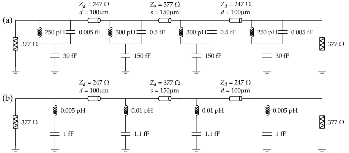
Figure 2.4. Circuit representation at 150 \mu\text{m} separation. Equivalent circuit model for the whole structure while working as a half-wave plate s = 150 \mu\text{m} . (a) Under y -polarised incidence, and (b) under x -polarised incidence. Here, Z_d , and Z_a are the characteristic impedance of the dielectric spacer and air, respectively, and d and s are the physical lengths of the equivalent transmission line sections corresponding to each 100 \mu\text{m} COC block, and 150 \mu\text{m} air gap between the blocks, respectively.
