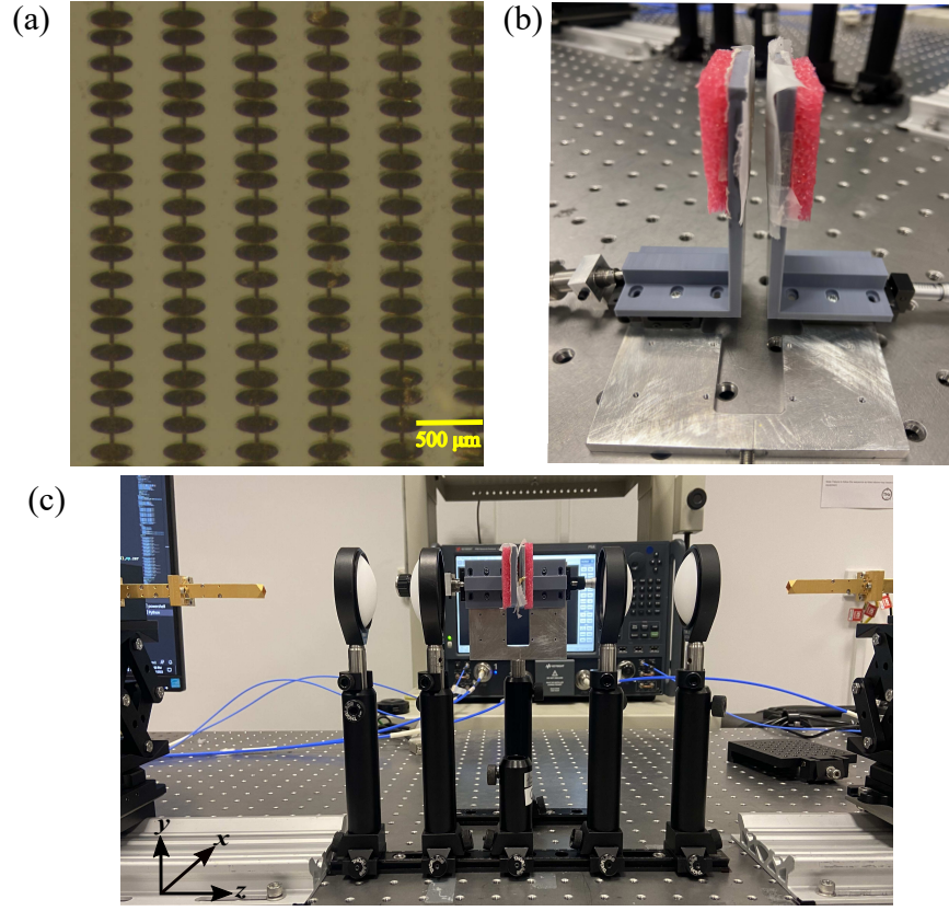
Figure 2.5. Metasurface sample and setup. Fabricated metasurface prototype and experimental setup. (a) Fabricated sample. (b) Sample pressed in the holder using low loss foam, and (c) measurement setup with four focusing lenses.
