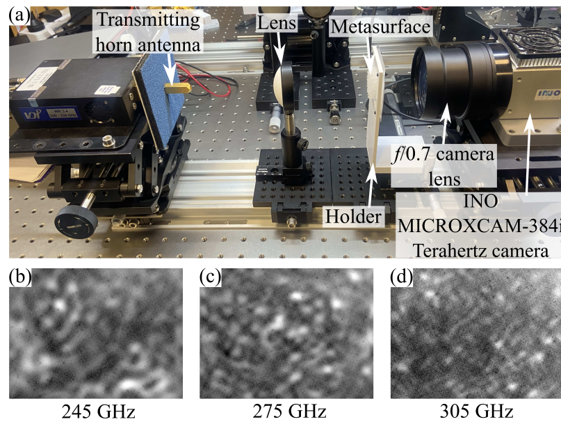
Figure 5.2. Experimental setup and representative wave patterns. Measurement setup and frequency-dependent near-field patterns. (a) Measurement setup with WR-3.4 source operating over 220–330 GHz, lens for collimation, pseudo-random metasurface on holder, and terahertz camera. (b), (c), and (d) Wave patterns at different frequencies 245 GHz, 275 GHz, and 305 GHz, respectively. These wave patterns correspond to a specific case: collimated wave input at a fixed distance and angle.
