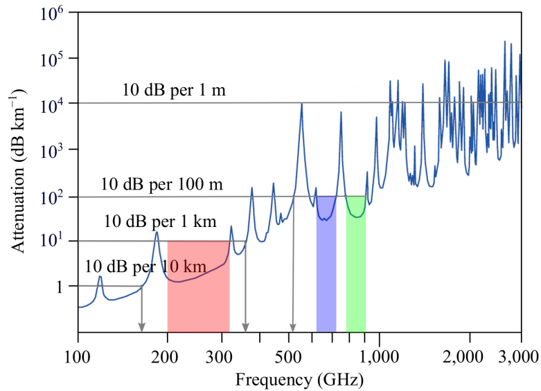
Figure 1.3. Frequency dependent atmospheric attenuation of terahertz waves. Attenuation of terahertz waves from 0.1 to 3 THz due to absorption by water-vapour in the atmosphere. Several resonance peaks disrupts the whole band, with 200–330 GHz (red) applicable for transmission over several kilometres, and 625–725 GHz (blue) and 780–910 GHz (green) optimal for indoor transmission. Adopted from Nagatsuma et al. (2016).
