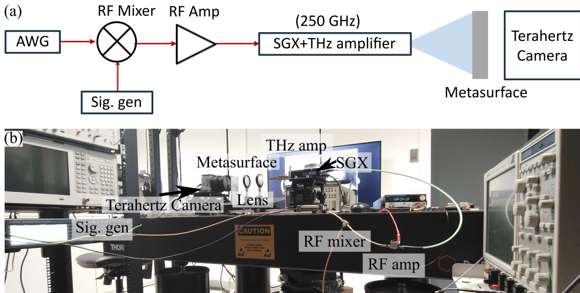
Figure 5.5. Finite-bandwidth measurement concept. (a) Block diagram of the finite-bandwidth terahertz measurement setup. (b) Measurement setup following the block diagram in (a). A two lens setup for convergent beam is shown as an example.
