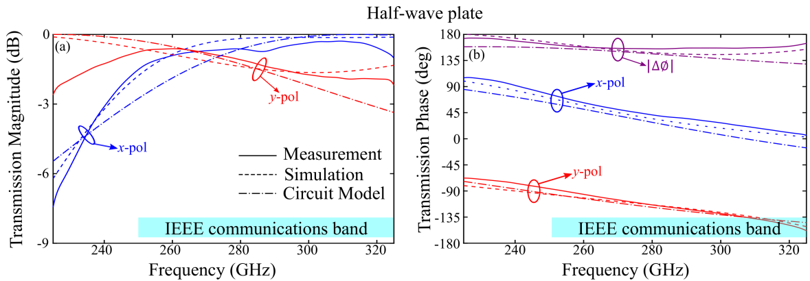
Figure 2.9. Half-wave plate simulated and measured transmission. Complex transmission coefficients of the metasurface at s = 150 \text{ } \mu\text{m} for x and y polarisation. (a) Magnitude, and (b) phase with phase difference |\Delta\phi| .
