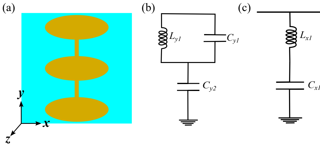
Figure 2.2. Circuit representation of metallic layers. Equivalent circuit model for each layer. (a) Metallic resonator. (b) Circuit models for y polarisation, and (c) x polarisation.
