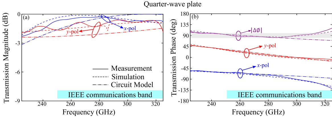
Figure 2.6. Quarter-wave plate simulated and measured transmission. Complex transmission coefficients of the metasurface at s = 0 \mu\text{m} for x and y polarisation. (a) Magnitude, and (b) phase with phase difference |\Delta\phi| . The region shaded in grey indicates the acceptable phase difference range around 90^\circ , corresponding to quarter-wave plate operation.
