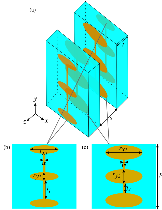
Figure 2.1. Metasurface structure. Schematic diagram of the polarisation conversion device. (a) Unit cell 3D view, (b) front metallic layer, and (c) back metallic layer. The geometric parameters of the design are r_{x1} = 240 \mu\text{m} , r_{x2} = 310 \mu\text{m} , r_{y1} = 70 \mu\text{m} , r_{y2} = 120 \mu\text{m} , w = 20 \mu\text{m} , l_1 = 155 \mu\text{m} , l_2 = 80 \mu\text{m} , p = 540 \mu\text{m} , t = 100 \mu\text{m} , and s is variable. Metallic resonators are made of gold to minimise metal loss and the substrate is cyclic olefin copolymer (COC) with a relative permittivity \epsilon_r = 2.33 and loss tangent \tan \delta = 0.0005 over the WR-3.4 band. Here, t denotes the thickness of each COC block. The two COC blocks forming the metasurface structure have identical thicknesses of 100 \mu\text{m} , while s represents the separation between them.
