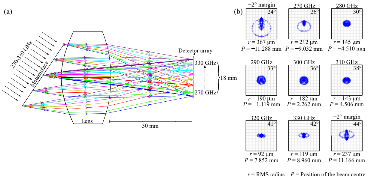
Figure 4.6. Focusing lens design and response. (a) Ray-tracing layout illustrating the input beam direction, object tilt and decentring, the optimised lens, and the corresponding beam focusing onto the image plane. (b) Corresponding ray-traced spot distributions on the image plane for incidence angles ranging from \pm 10^\circ relative to the lens optical axis, including a \pm 2^\circ margin to account for alignment tolerances, as indicated by the blue markers. These angles correspond to metasurface beam deflection angles of 64^\circ – 48^\circ before tilt, representing frequencies from 270–330 GHz, as shown in Fig. 4.5(b). Including the \pm 2^\circ margin, the angular range extends to 66^\circ – 46^\circ . The RMS spot radius, r , and focal position on the image plane, P , are indicated. The RMS spot sizes are derived from geometric ray-tracing and do not include diffraction effects. The lens optimisation therefore aims to achieve tight geometric focusing while maintaining a focal position separation in mm-scale to accommodate diffraction-limited spot sizes at terahertz frequencies.
