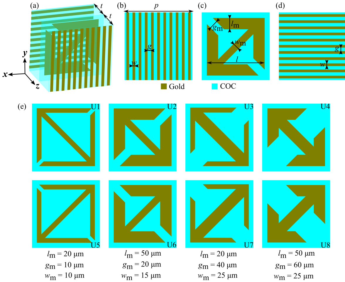
Figure 4.3. Unit cell design architecture. Schematic diagram of a unit cell. (a) Unit cell 3D view, (b) front wire-grid layer, (c) middle resonant layer, and (d) back wire-grid layer. The geometric parameters of the design are t = 65 \mu\text{m} , w = 6 \mu\text{m} , g = 8 \mu\text{m} , l = 130 \mu\text{m} , and p = 154 \mu\text{m} . The parameters l_m , w_m , and g_m are variable to control the output phase. (e) Designs and the parametric variations of the middle resonator used to control phase response. Metallic resonators are made of gold to minimise metal loss and the substrate is cyclic olefin copolymer (COC) with a relative permittivity \epsilon_r = 2.34 and loss tangent \tan \delta = 0.0005 . U1–U8 denote the different middle resonant structure designs, where U5–U8 are the mirror images of U1–U4 about the vertical axis, respectively.
