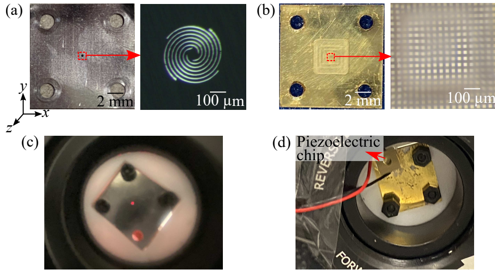
Figure 3.5. Device structure and integration. Fabricated sample and device assembly. (a) Fabricated niobium (Nb) spiral structure, showing the extended Nb plate and four screw holes with a microscopic view of the central spiral. (b) Optical image of the COC-gold plane with screw holes at corners and air-cavity at the centre, also showing a microscopic view of the periodic square apertured gold structure visible through the transparent COC. (c) Front view (Nb side) of the fully assembled device fastened with nuts and bolts and mounted onto a sample holder. (d) Backside view (gold side) of the assembled device, showing the mounted piezoelectric chip attached to one corner of the gold plane.
