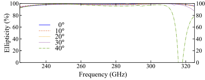
Figure 2.8. Angular stability of the quarter-wave plate under oblique incidence. Simulated ellipticity of the quarter-wave plate under oblique incidence for incidence angles ranging from 0^\circ to 40^\circ . The device maintains an ellipticity above 95% up to approximately 30^\circ incidence across most of the operation band, demonstrating good angular stability.
