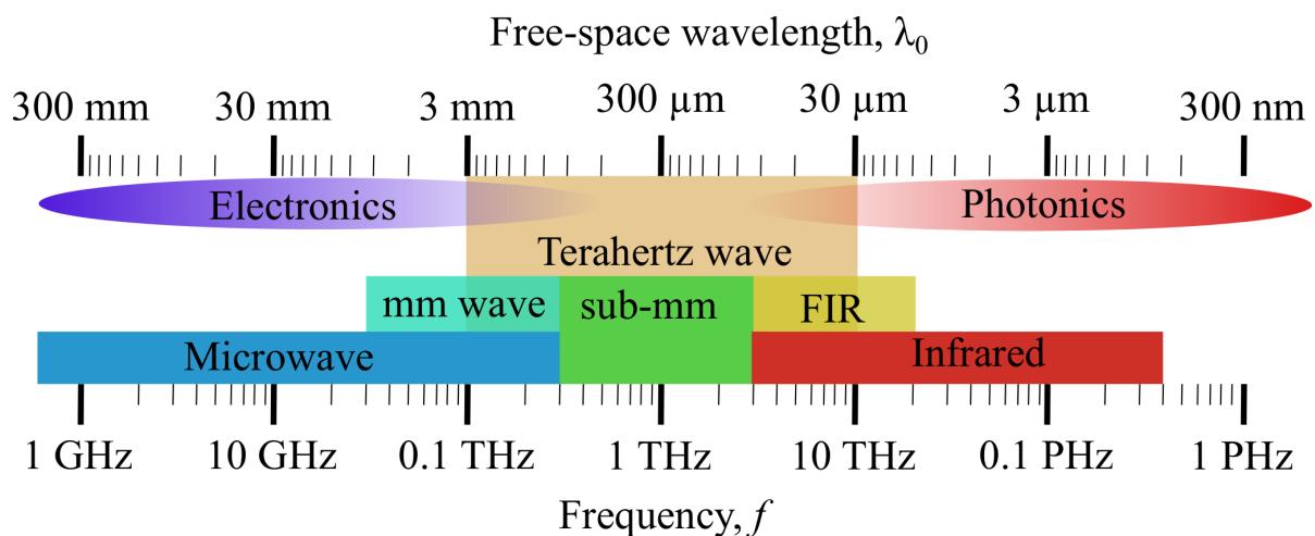
Figure 1.1. Electromagnetic spectrum. The terahertz frequency range within the electromagnetic spectrum, situated between the microwave and infrared waves and overlapping with the millimetre wave, sub-millimetre wave and far-infrared region. The figure highlights the gradual fading of electronic and photonic generation techniques in the terahertz regime.
