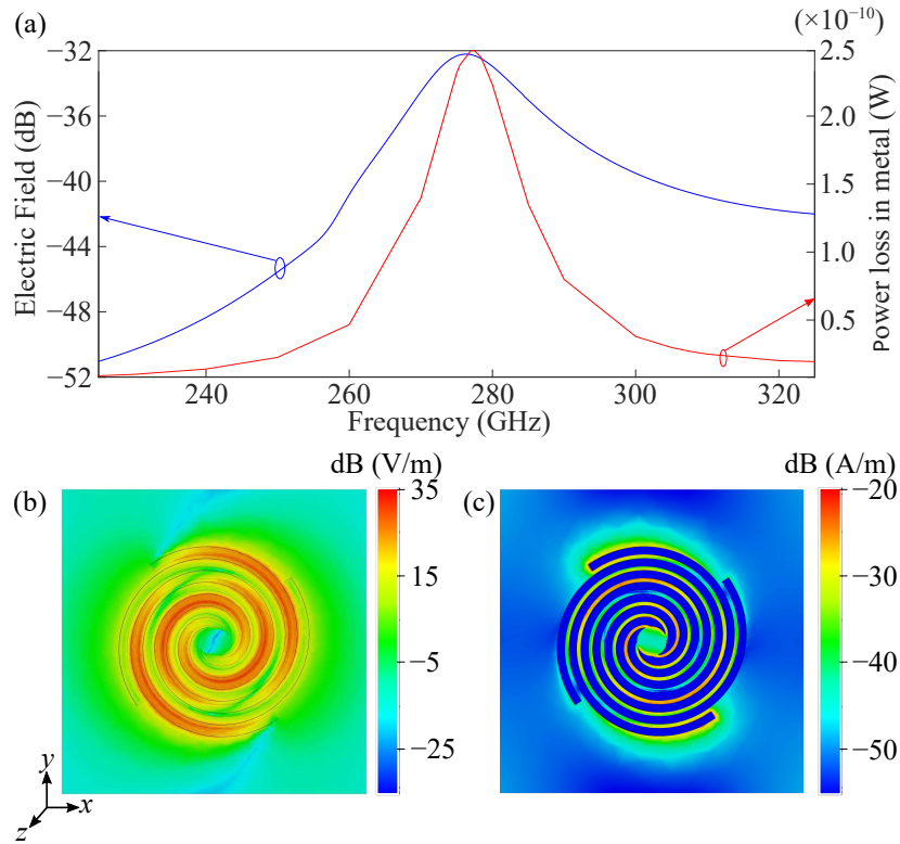
Figure 3.2. Electromagnetic simulation results. Electromagnetic response of the proposed terahertz bolometer. (a) Frequency-dependent electric field enhancement at the centre of the spiral, and frequency-dependent power loss in niobium metal including niobium spiral. (b) Electric field intensity, and (c) surface current profile at 277.5 GHz. The incident wave is linearly polarised and propagates in the -z -direction.
