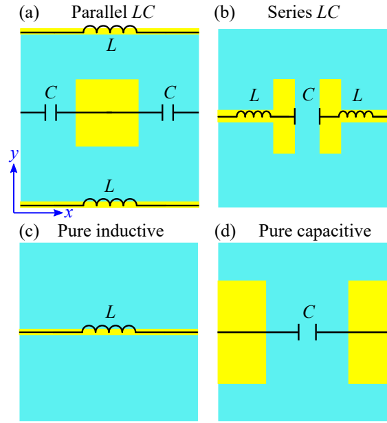
Figure 1.5. Equivalent circuit interpretation of metasurface unit cell geometries. Representative metallic patterns and their corresponding equivalent circuit interpretations under x -polarised incidence. a) Parallel LC, (b) series LC, (c) predominantly inductive, and (d) predominantly capacitive responses. The effective inductance is primarily governed by the current path length, and effective capacitance is determined by gaps or closely spaced conductors. Such equivalent circuit representations provide physical insight into the resonant behaviour of metasurfaces and enable prediction of resonance arising from inductive and capacitive reactance. Adopted from You et al. (2022).
