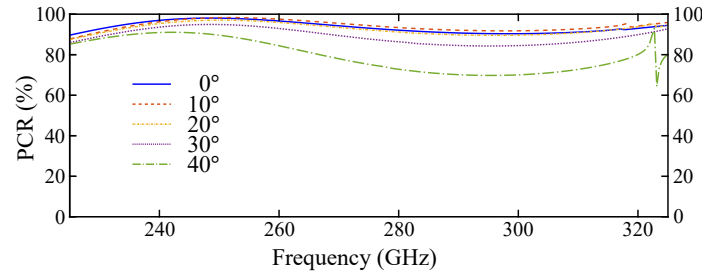
Figure 2.11. Angular stability of the half-wave plate under oblique incidence. Simulated polarisation conversion ratio of the half-wave plate under oblique incidence for incidence angles ranging from 0^\circ to 40^\circ . The device maintains a PCR above 80% up to approximately 30^\circ incidence across most of the operation band, demonstrating good angular stability.
