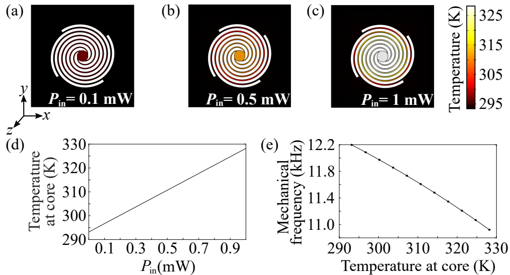
Figure 3.4. Thermomechanical simulation results. COMSOL Multiphysics simulation results illustrating the thermal and mechanical response of the niobium spiral bolometer. (a–c) Simulated heat maps showing temperature distribution at input powers of (a) 0.1 mW, (b) 0.5 mW, and (c) 1 mW, respectively. (d) Plot of input power, P_{in} , versus temperature at the core of the spiral, indicating a linear rise from 293 K to approximately 328 K. (e) Corresponding mechanical resonance frequency as a function of core temperature.
