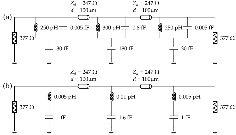
Figure 2.3. Circuit representation at 0 \mu\text{m} separation. Equivalent circuit model for the whole structure while working as a quarter-wave plate s = 0 \mu\text{m} . (a) Under y -polarised incidence, and (b) under x -polarised incidence. Here, Z_d is the characteristic impedance of the dielectric spacer, and d is the physical length of the equivalent transmission line section corresponding to each 100 \mu\text{m} COC block.
