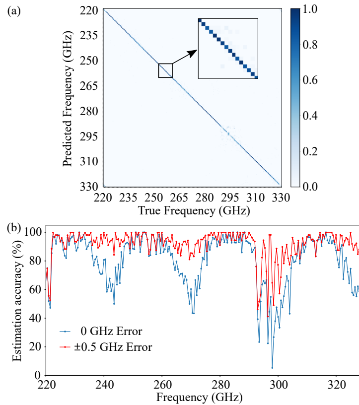
Figure 5.3. Metasurface and CNN performance. Frequency estimation performance of the pseudo-random metasurface across the 220–330 GHz band. (a) Confusion matrix of predicted versus true frequencies. (b) Estimation accuracy at 0.5 GHz frequency resolution, with 0 GHz error (blue) indicating exact predictions and \pm 0.5 GHz error (red) showing predictions within 1 GHz tolerance.
