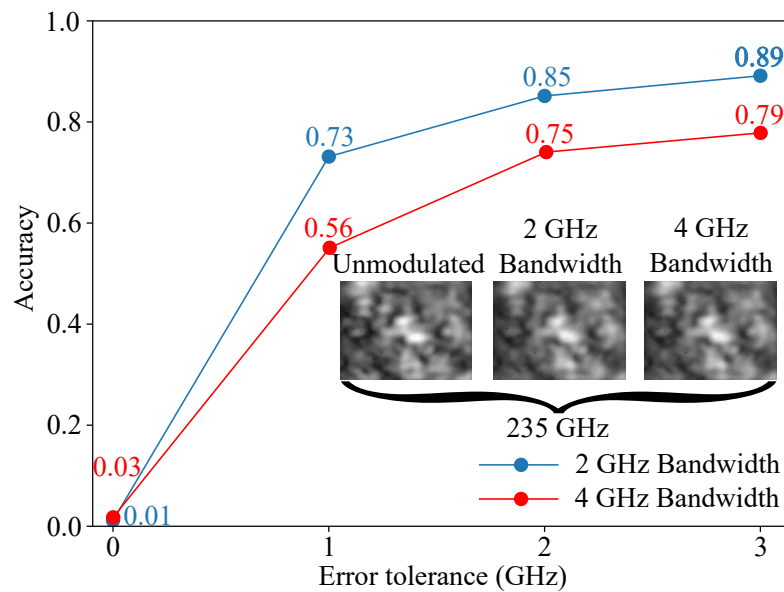
Figure 5.6. Accuracy under finite-bandwidth wave. Frequency estimation accuracy with respect to error tolerance for modulated signals with 2 GHz bandwidth (blue), and 4 GHz bandwidth (red). Insets show representative near-field patterns at 235 GHz for unmodulated, 2 GHz, and 4 GHz bandwidth signals.
