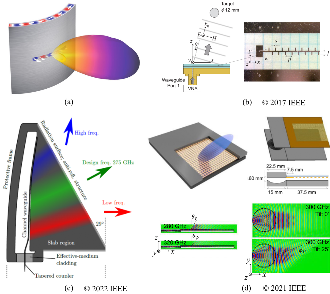
Figure 1.10. Terahertz leaky-wave antennas. (a) Parallel-plate waveguide-based LWA. A rectangular slot is cut on one side of the waveguide to allow continuous radiation (Gueboukha et al. , 2023). (b) Microstrip line-based LWA. Periodical gratings are constructed along the microstrip line to allow wave leakage into free-space (Murano et al. , 2017). (c) Dielectric channel waveguide-based LWA. The separation distance between the channel waveguide and the dielectric slab gradually changed, allowing the leakage energy enter the silicon slab from different directions for different frequencies (Headland and Withayachumnankul, 2022). (d) 2-D LWA. Beam steering with one dimension is controlled by frequency, while the other dimension is controlled by mechanically rotating the source position along a Lundberg lens. Adapted from Sato and Monnai (2021).
