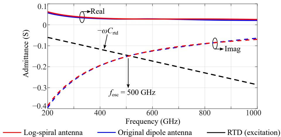
Figure 3.3. Comparison of Y-parameters simulated from the original dipole antenna and RTD with a log-spiral antenna. The oscillation frequency is at the crossing point where the negative susceptance of the RTD excitation balances the susceptance of the antennas.
