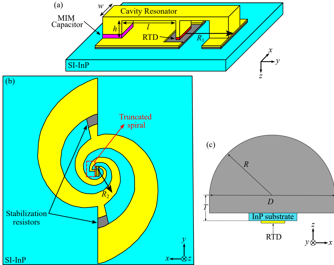
Figure 3.1. CP RTD structure. (a) Cavity-resonator-coupled RTD schematic. The rectangular cavity with length l , width w and height h helps improve the output power. R_1 refers to the inner radius of the log-spiral antenna intended for radiation. (b) Cavity-coupled RTD with spiral bias connections. R_2 refers to the outer radius of the log-spiral antenna. (c) RTD with a hyper-hemispherical silicon lens to collimate the output wavefront. The silicon lens has a diameter of D = 2R and an extended thickness of T , which includes the InP substrate thickness.
