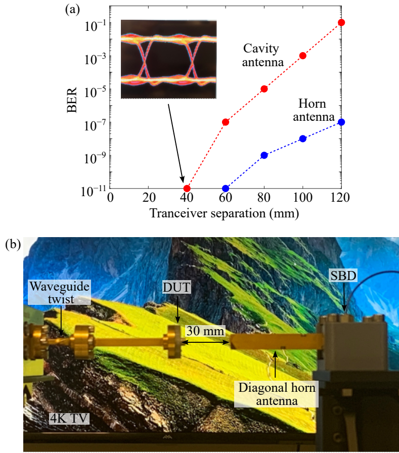
Figure 5.11. Communications measurement results. (a) Measured BER as a function of transceiver separation distances. The inset shows the eye diagram at the distance of 40 mm. (b) 4K-resolution video transmission demonstration. The cavity antenna with a waveguide twist is placed at the left as the transmitter and the SBD with a diagonal horn is placed at the right for envelope detection. The waveguide twist helps aligning the E -field with the SBD. The background depicts a static image of a successful video transmission.
