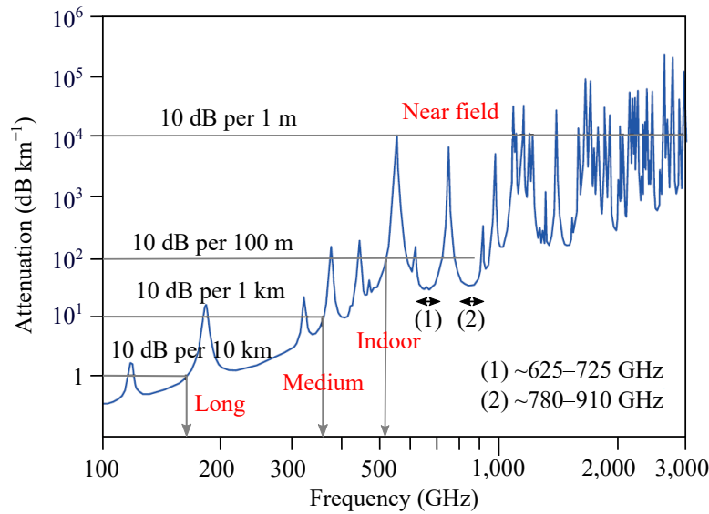
Figure 1.1. Atmospheric attenuation. Attenuation of electromagnetic waves by the atmosphere. Two transmission windows above 600 GHz include ~625–725 GHz and ~780–910 GHz. Adopted from Nagatsuma et al. (2016).
