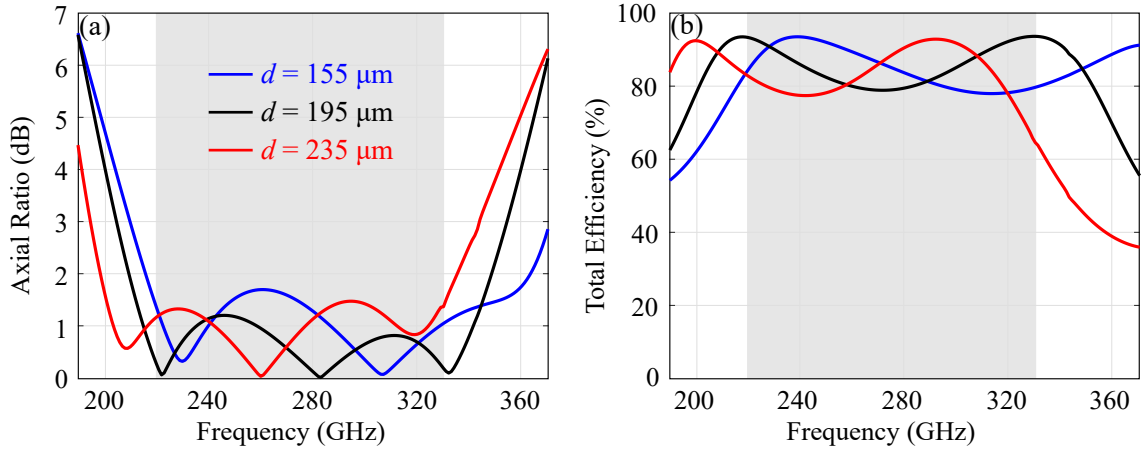
Figure 5.7. Simulated performance of the quarter-wave transmitarray with different spacer thicknesses. (a) Axial ratio and (b) total efficiency. The shaded area marks the frequency range of interest from 220 GHz to 330 GHz.
