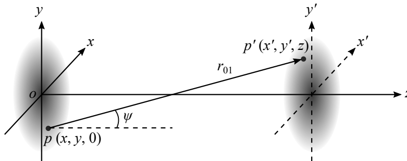
Figure 2.1. Huygens-Fresnel principle solution space. A diffracting aperture is located in (x, y, 0) plane, while field distributions that require to be calculated reside in (x', y', z) plane. Points p and p' are for illustration purpose and they are randomly taken from the diffracting aperture and observation plane, respectively. The distance between p and p' is represented by r_{01} , and \psi denotes the angle between pp' -line and the z -axis. Adapted from Headland (2017).
