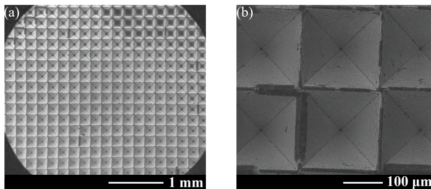
Figure 8.4. Scanning electron micrographs of the fabricated absorber. (a) Partial view and (b) magnified view containing 6 unit cells.
