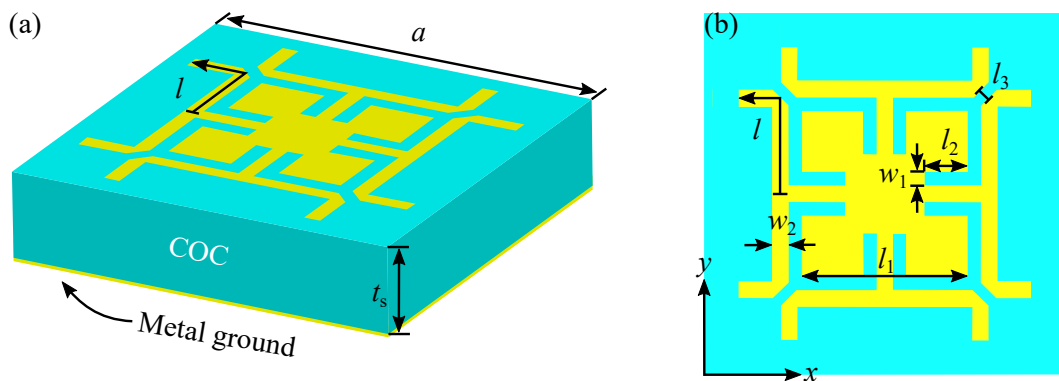
Figure 3.2. Unit cell geometry. (a) 3D view, and (b) top view. The detailed dimensions are as follows: a = 120 \mu\text{m} , t_s = 36 \mu\text{m} , l_1 = 55 \mu\text{m} , l_2 = 14.5 \mu\text{m} , l_3 = 3\sqrt{2} \mu\text{m} , w_1 = w_2 = 5 \mu\text{m} , and l denotes the varying stub length.
