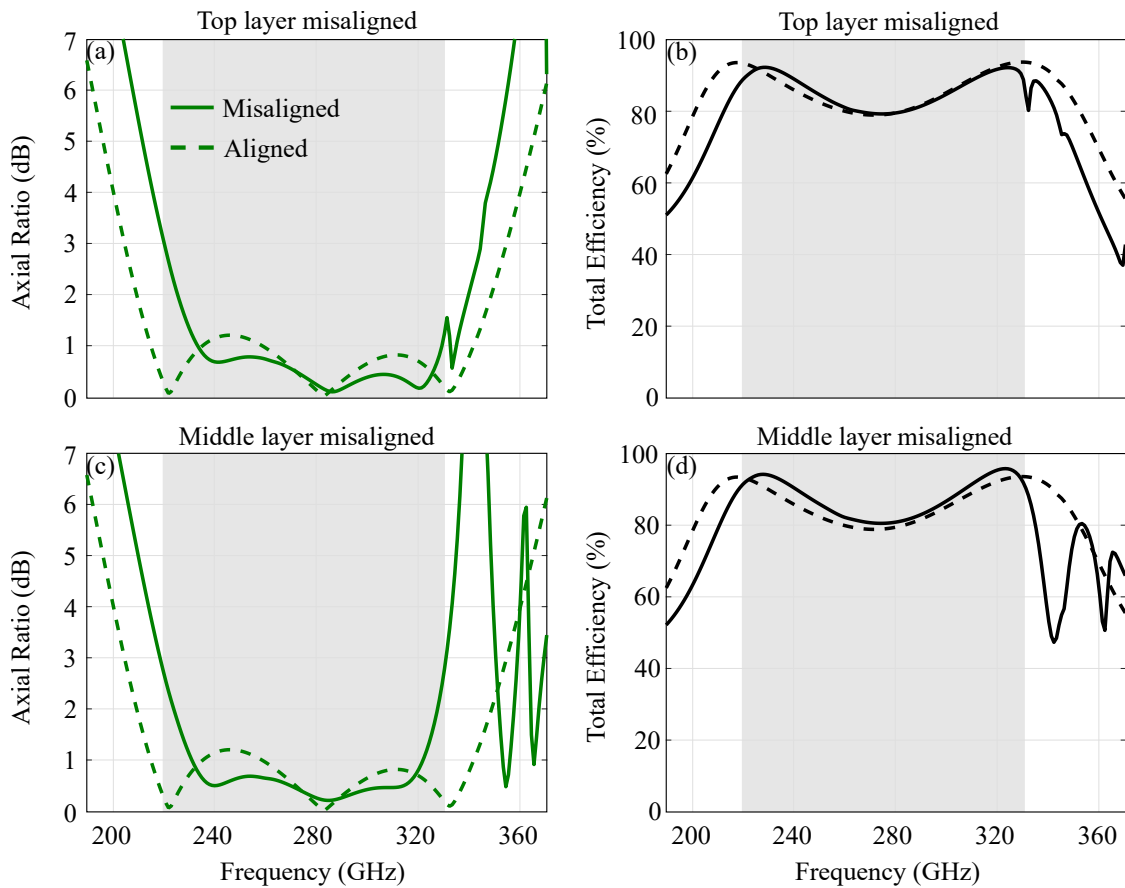
Figure 5.9. Simulated axial ratio and total efficiency of the quarter-wave transmitarray with and without misalignment. [(a, b)] Top layer shifts along the x - and y -axes are both 200\ \mu\text{m} (37% of the unit cell size). [(c, d)] Middle layer shifts along the x - and y -axes are both 120\ \mu\text{m} (22% of the unit cell size). The shaded area marks the frequency range of interest from 220 GHz to 330 GHz.
