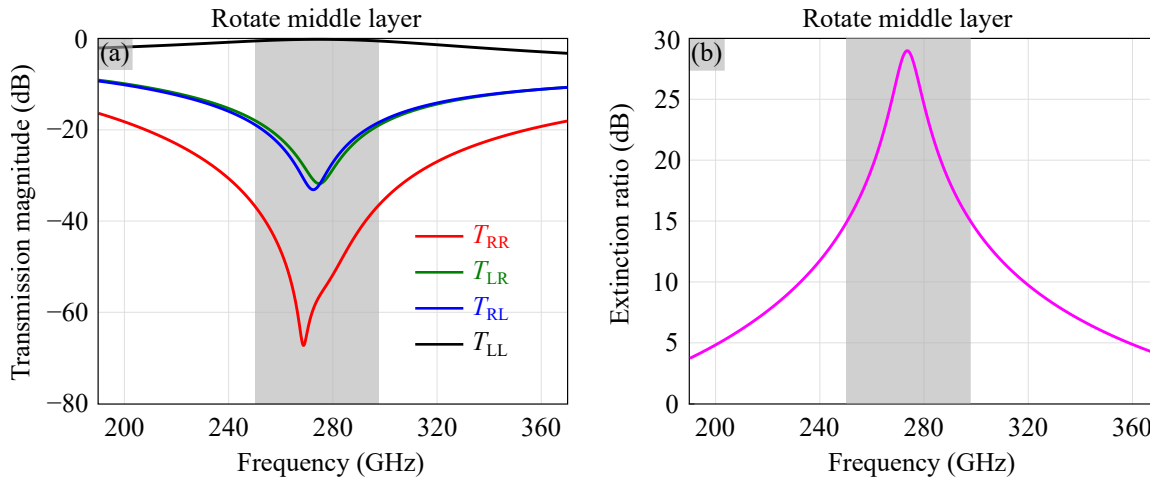
Figure 7.6. Simulation results of the proposed structure functioning as a circular polariser that allows LHCP waves transmission. (a) Transmission magnitude and (b) extinction ratio. The middle metallic layer is rotated by 90^\circ around the z -axis. The extinction ratio here is defined as the transmittance ratio |T_{LL}|^2 / (|T_{RL}|^2 + |T_{LR}|^2 + |T_{RR}|^2) . The simulation curves in (a, b) are identical to the simulation ones shown in Figure 7.3, while the only difference is the polarisation exchange between RHCP and LHCP. The shaded area marks the 15-dB extinction ratio bandwidth from 251 GHz to 298 GHz.
