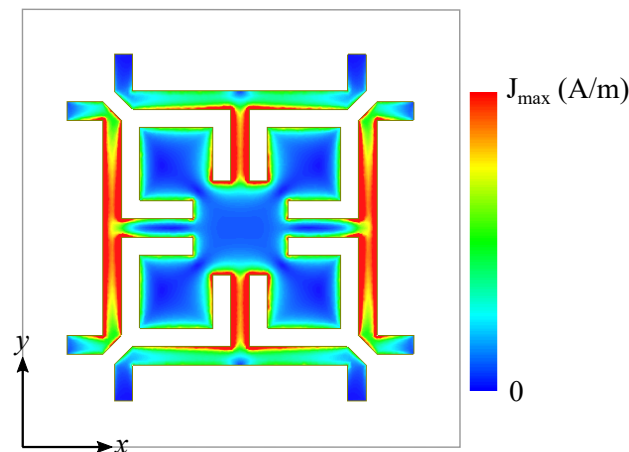
Figure 3.3. Top resonator surface currents distribution. Surface currents distribution on the top resonator under a normally-incident y -polarised excitation at 1.00 THz with l = 44.5\text{ }\mu\text{m} . The current is in linear scale and the outline box defines the unit cell size.
