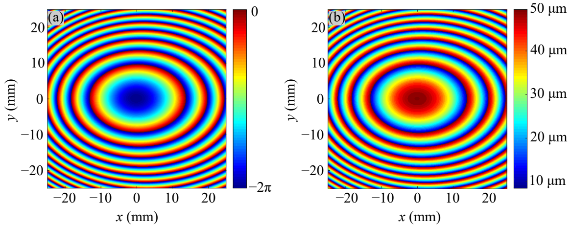
Figure 3.7. Distributions of desired phase response and stub length on the reflectarray surface for beam focusing. (a) Phase distribution and (b) stub length distribution.
