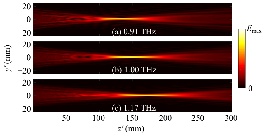
Figure 3.8. Frequency-dependent beam focusing operations. Calculated linear field distributions along propagation with a TM-polarised plane wave excitation at (a) 0.91 THz, (b) 1.00 THz, and (c) 1.17 THz.
