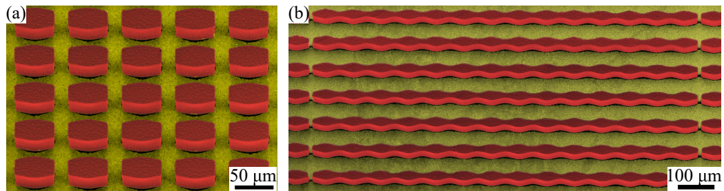
Figure 1.5. Reflectarray-based reflective waveplates made of identical dielectric resonators. (a) Quarter-wave mirror. (b) Half-wave mirror. Adopted from Lee et al. (2018a).
