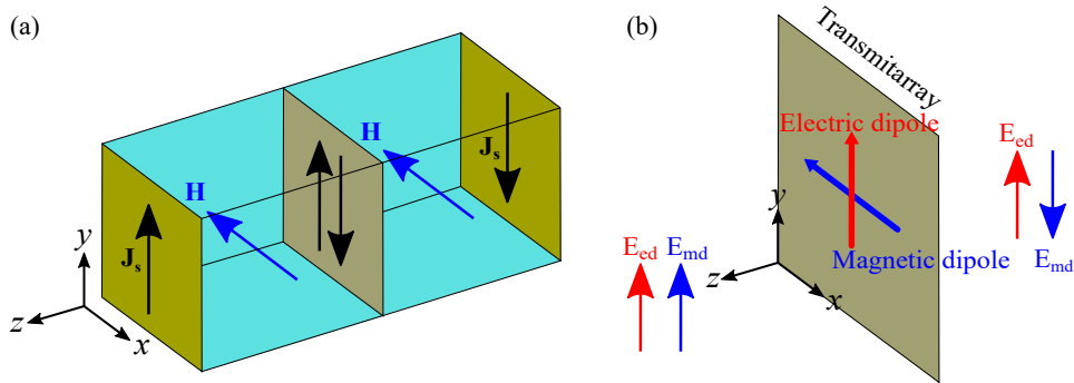
Figure 5.1. Induced currents and electric field distributions of the transmitarray. (a) Schematic diagram of the induced currents on the transmitarray generated by a quasi-static magnetic field along the -x -axis. The top and bottom layers are identical, and the dielectric spacers share the same thickness. (b) Sketch of the electric field distributions contributed from the electric and magnetic dipoles of equal strength.
